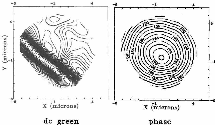
Figure 1: Green reflectance map (left) and phase map (right) obtained on a sample of bulk gold (modulation frequency : 1 MHz). A surface scratch clearly appears on the reflectance map, but does not perturb the phase of the photothermal signal.
