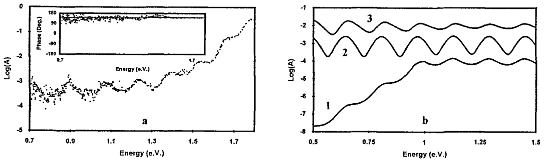
Figure 2 : (a) Calibrated experimental A(h\nu) spectra obtained from PDS data with front ( \Delta ) and rear (o) illumination for an \alpha -Si:H film ( d \simeq 1 \mu\text{m} ) (the phase of the PDS signal is reported in the inset); (b) computed A(h\nu) spectra for a homogeneous film ( d = 1 \mu\text{m} ) with \alpha = 1 \text{ cm}^{-1} for h\nu \geq 1 \text{ eV} and \alpha decreasing from 1 \text{ cm}^{-1} to 10^{-4} \text{ cm}^{-1} for 0.5 \leq h\nu \leq 1 \text{ eV} (1) and for a similar film (total d = 1 \mu\text{m} ) including a surface layer with \alpha_s = 10^3 \text{ cm}^{-1} and d_s = 10 (2), 100 (3) nm.
