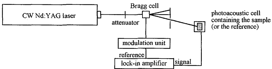
Figure 1: scheme of the photoacoustics experiment
