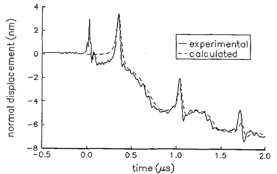
Figure 5 Experimental and calculated normal displacements vs time for a large spot size
