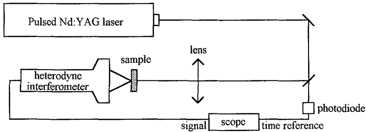
Figure 3: scheme of the laser-ultrasonics experiment
