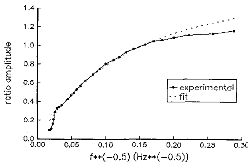
Figure 2: comparison of the experimental and fitted ratio amplitude curves
