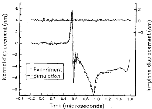
Figure 10: Theoretical and experimental normal and in-plane displacement curves vs time at equal distance from two epicenters (as expected, the experimental in-plane displacement is zero).
