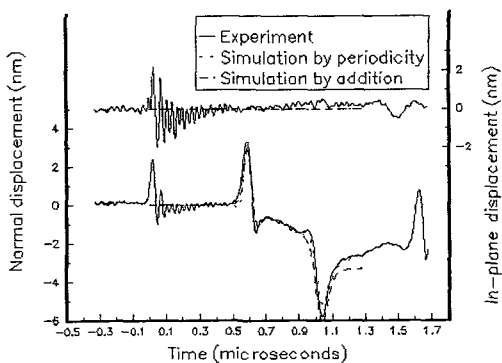
Figure 8: Theoretical and experimental normal and in-plane displacement curves vs time at equal distance from two epicenters (as expected, the experimental in-plane displacement is zero)
