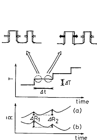
Fig.3 Schematic explanation of the simultaneous coarsening and dissolution.
