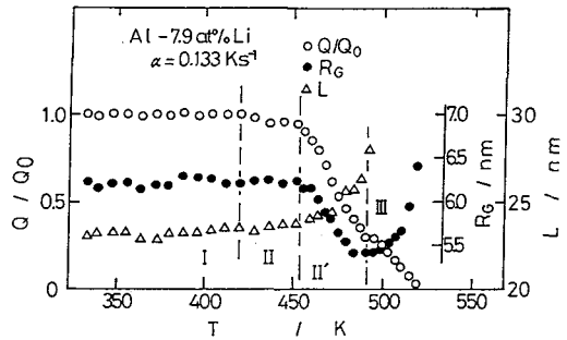
Fig.2 Change in the Guinier radius, the normalized integrated intensity, and the interparticle distance. Heat treatment is the same as Fig.1.
