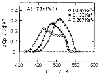
Fig.1 Change of the specific heat for Al-7.9 at%Li aged at 423K for 86.4ks.
