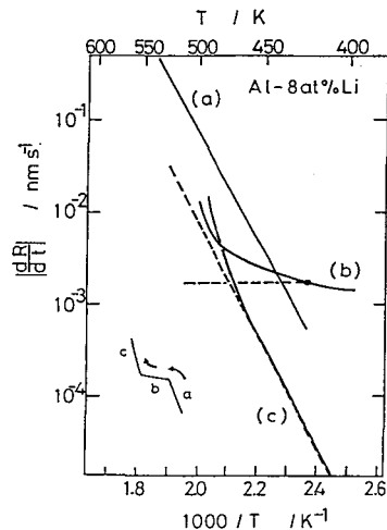
Fig.4 Evaluate of the change in the radius due to (a)dissolution, (b)dissolution driving force, and (c)coarsening
