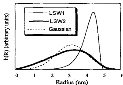
Fig 1: Gaussian and LSW's distributions for a FeCu1.5% irradiated 4.7 C/cm 2 at 300 °C .
