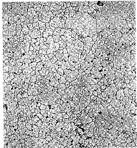
Figure 4 : Sprayed INCONEL 625 structure after heat-treatment
