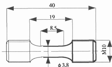
Figure 10 : Morphology of the LCF specimens
