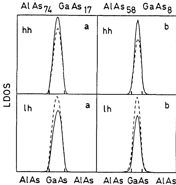
Figure 2 : Spatial distribution of the amplitudes of the p_x component (dashed line) and p_y component (solid line) for the first hh and lh levels of the samples \text{AlAs}_{74}\text{GaAs}_{17} (a) and \text{AlAs}_{58}\text{GaAs}_8 (b).
