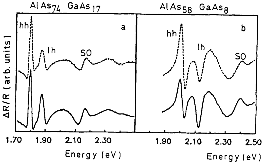
Figure 1 : Piezoreflectance spectra of the AlAs 74 GaAs 17 (a) and AlAs 58 GaAs 8 (b) superlattices obtained at 80K, with light polarized parallel to [011] (solid line) and parallel to [233] (dashed line).
