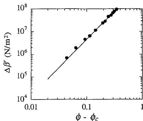
Fig. 9: Critical scaling behavior of the additional modulus of the droplet network phase of the 25-Å radius microemulsions in hexane at high frequencies, when it forms a random rigid network. The exponent is \tau \approx 2.5 and the critical volume fraction is \phi_c \approx 0.16 .
