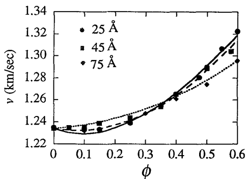
Fig. 6: The velocity of sound for AOT-decane-water microemulsions of three different radii, 25, 45 and 75 Å, as a function of volume fraction. The solid lines represent fits to the effective medium model.
