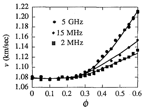
Fig. 7: Velocity of sound in 25-Å radius AOT-hexane-water microemulsions as a function of volume fraction for different frequencies. The solid lines represent fits to the effective medium model, treating the droplet phase as a random, connected medium that can support shear.
