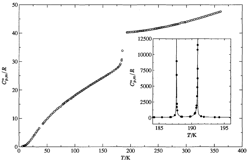
Fig. 1. — Low-temperature heat capacity of tetraethoxysilane.
