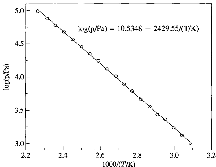
Fig. 2. — Vapour pressure of tetraethoxysilane from 323 to 441 K.
