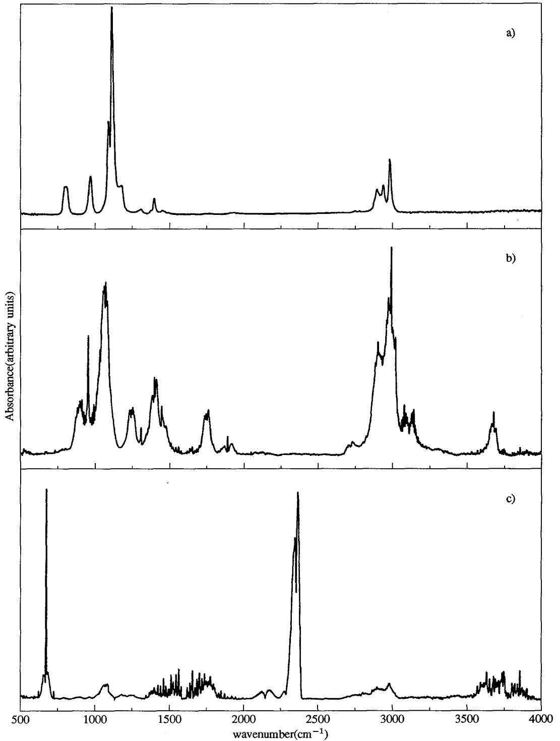
Fig. 3. — Infrared spectra of a) TEOS, b) product spectrum of pyrolysis at low pressure, and c) product spectrum of pyrolysis at atmospheric pressure in oxygen.
