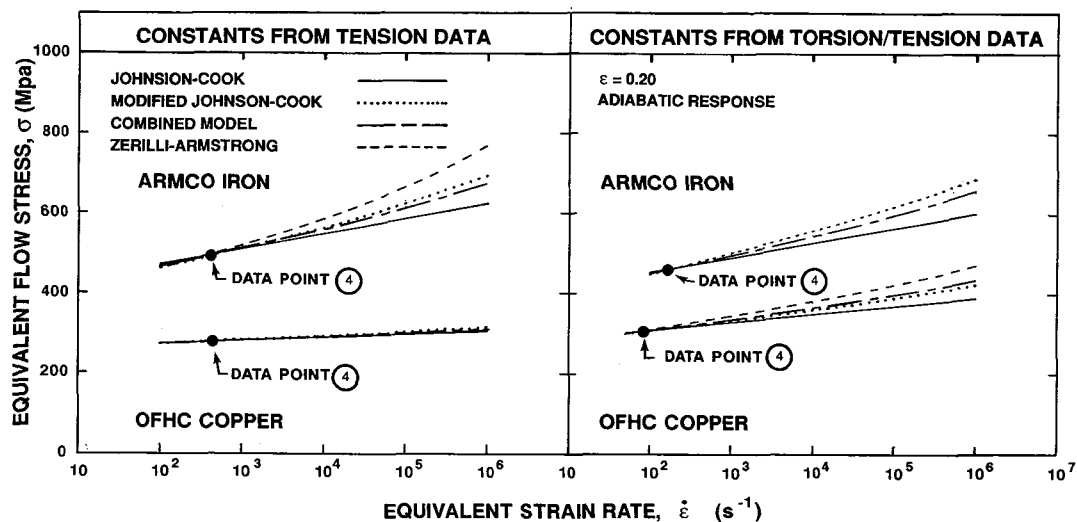
Figure 3. Stress-strain rate relationships for OFHC copper and Armco iron, using various models and constants
