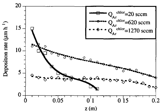
Fig. 11. — Experimental deposition rates versus location on the substrate with the carrying \text{ZrCl}_4 argon flow rate increased to 1270 sccm. The substrate was in contact in this case with the separating tube.
