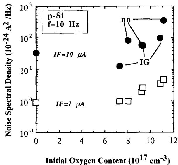
Fig. 9. — Correlation between the current noise spectral density measured at f = 10 Hz and the initial oxygen content of the substrates used for the fabrication of the n^+p diodes. The noise is measured at two different current levels.
