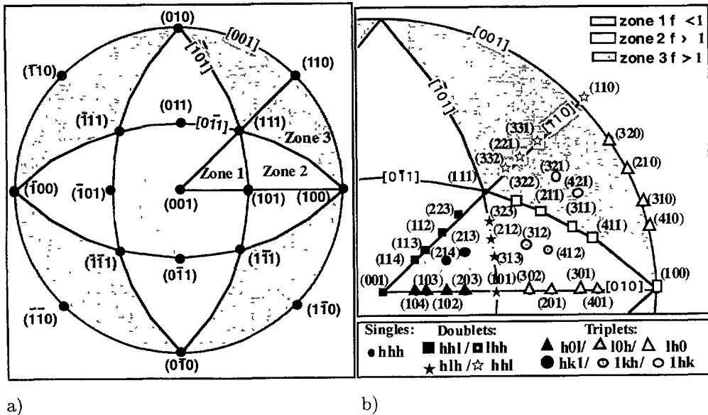
Fig. 14. — Dissymmetry factor of the diffraction lines represented in the (001) stereographic projection of the BaTiO 3 structure: a) whole projection; b) focused projection of the non equivalent hkl lines
