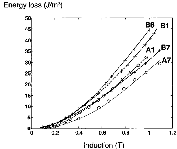
Fig. 3. — Total losses at 10 kHz vs. induction for classical and rapid annealing (○)→ A alloy, (+)→ B alloy.
