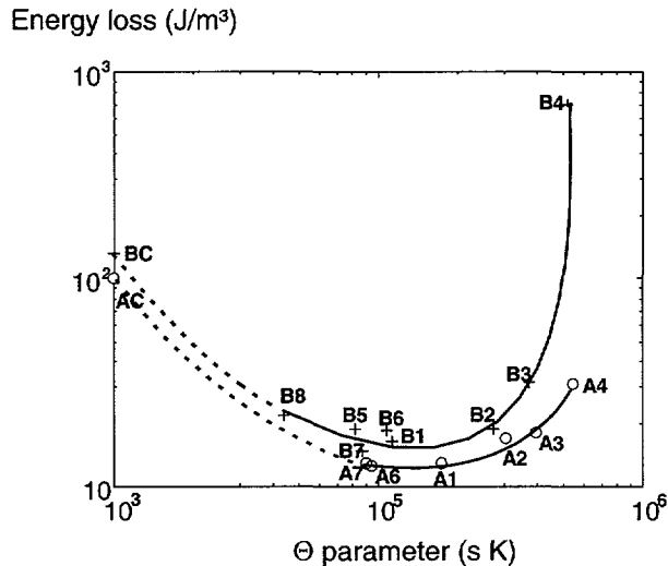
Fig. 2. — Electromagnetic losses at 1 kHz, 0.8 T as function of \Theta parameter ( \circ ) \rightarrow A alloy, (+) \rightarrow B alloy.
