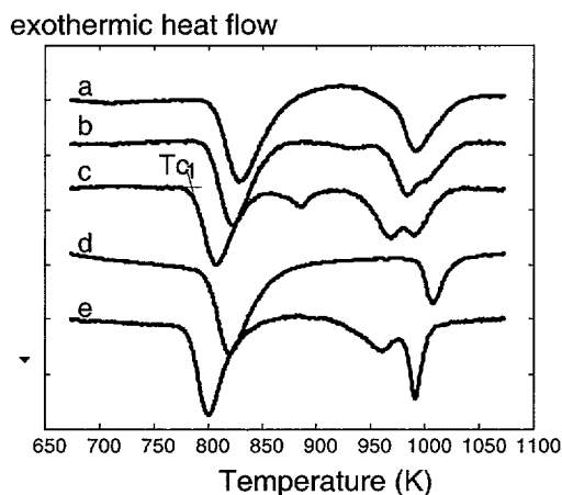
Fig. 1. — ATD plots obtained during continuous heating at rate of 40 (a), 20 (b) and 10 K/min (c) on as cast B sample, 40 (d) and 10 K/min (e) on as cast A sample.
