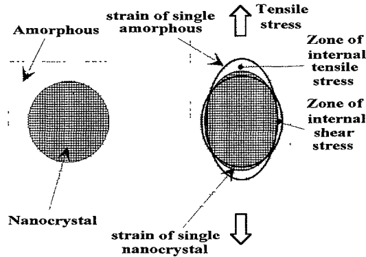
Fig. 4. — Origin of internal stresses induced by external tensile stress.
