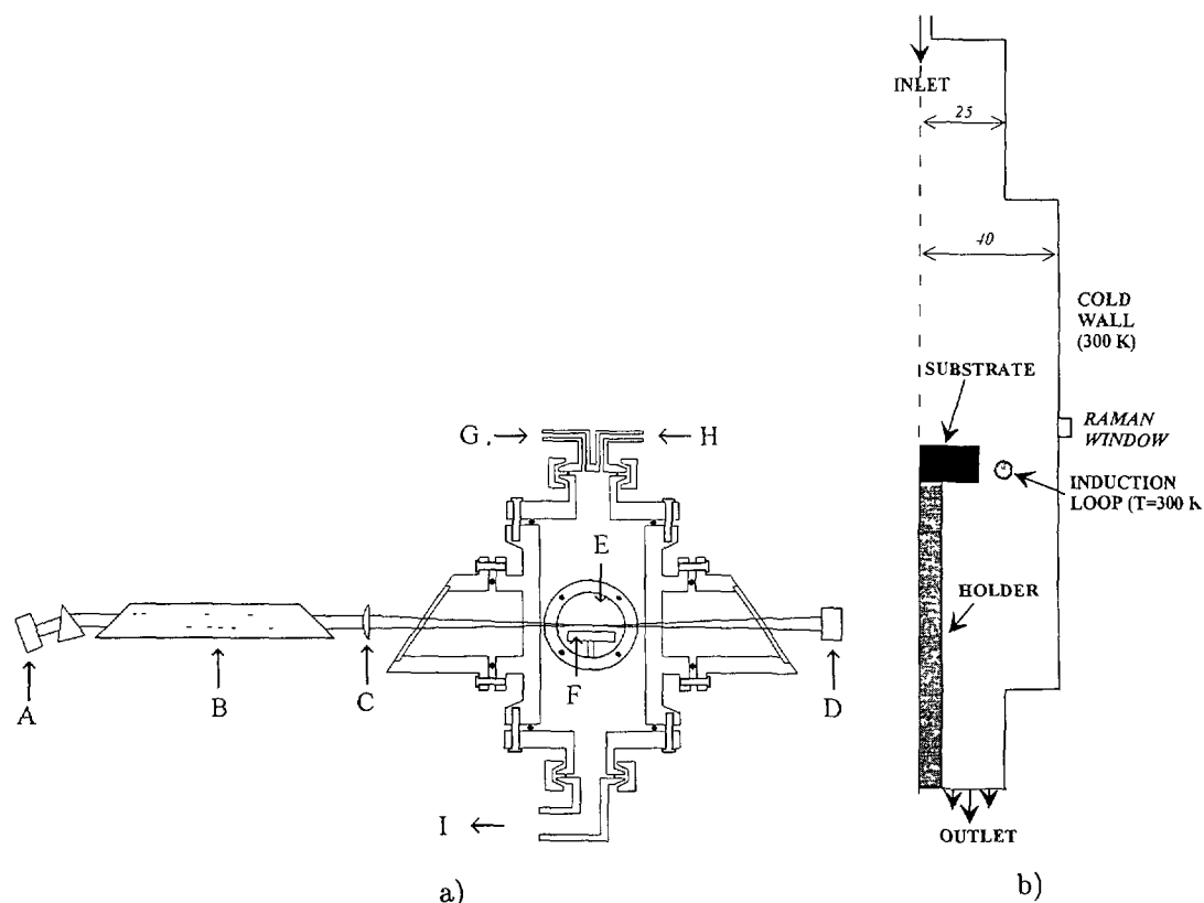
Fig. 1. — a) Cross section of the reactor: A - Plane mirror. B - Laser tube. C - Lens f = 0.20 m. D - Spherical mirror R = 0.20 m. E - Ca F 2 windows. F - Graphite substrate. G - Gas mixture inlet. H - Pressure measurement. I - Exit. b) Schematic representation for modelling studies (dimensions are in mm).
