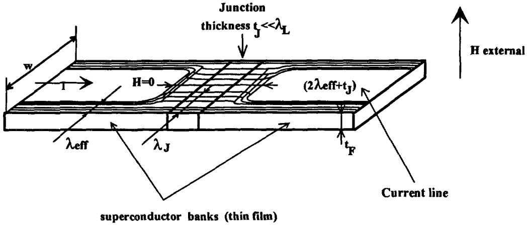
Fig. 1. — Sketch view of electrical and geometrical parameters implied in a Josephson junction.
