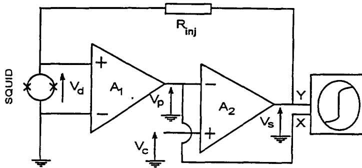
Fig. 8. — Sketch view of the voltage biasing circuit.
