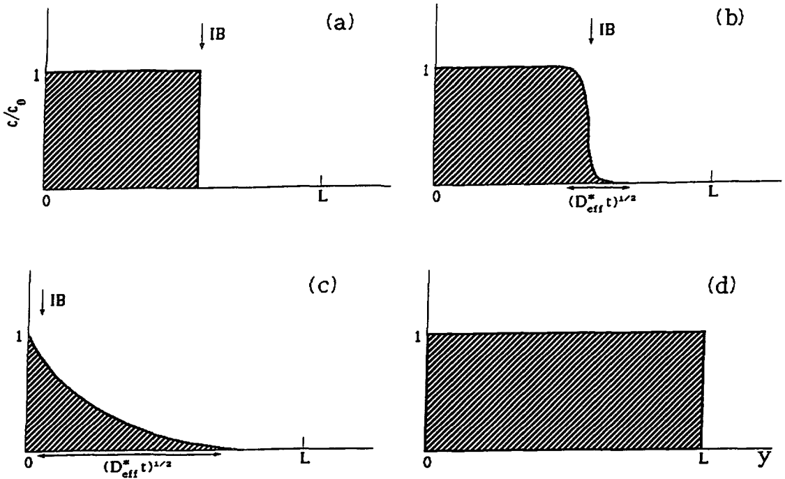
Fig. 2. — Schematic 18 O penetration profiles under the A-regime conditions. a) idealized and b) more realistic profile for the drift regime ; c) pure diffusion regime ; d) full isotope equilibrium.
