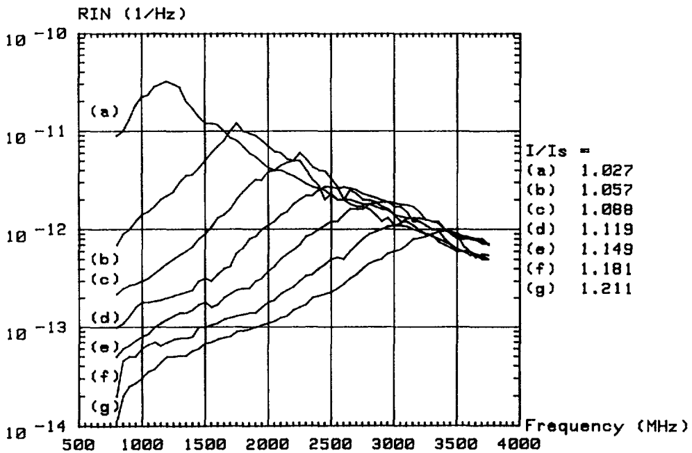
Fig. 7. — RIN versus frequency for different values of injection current.
