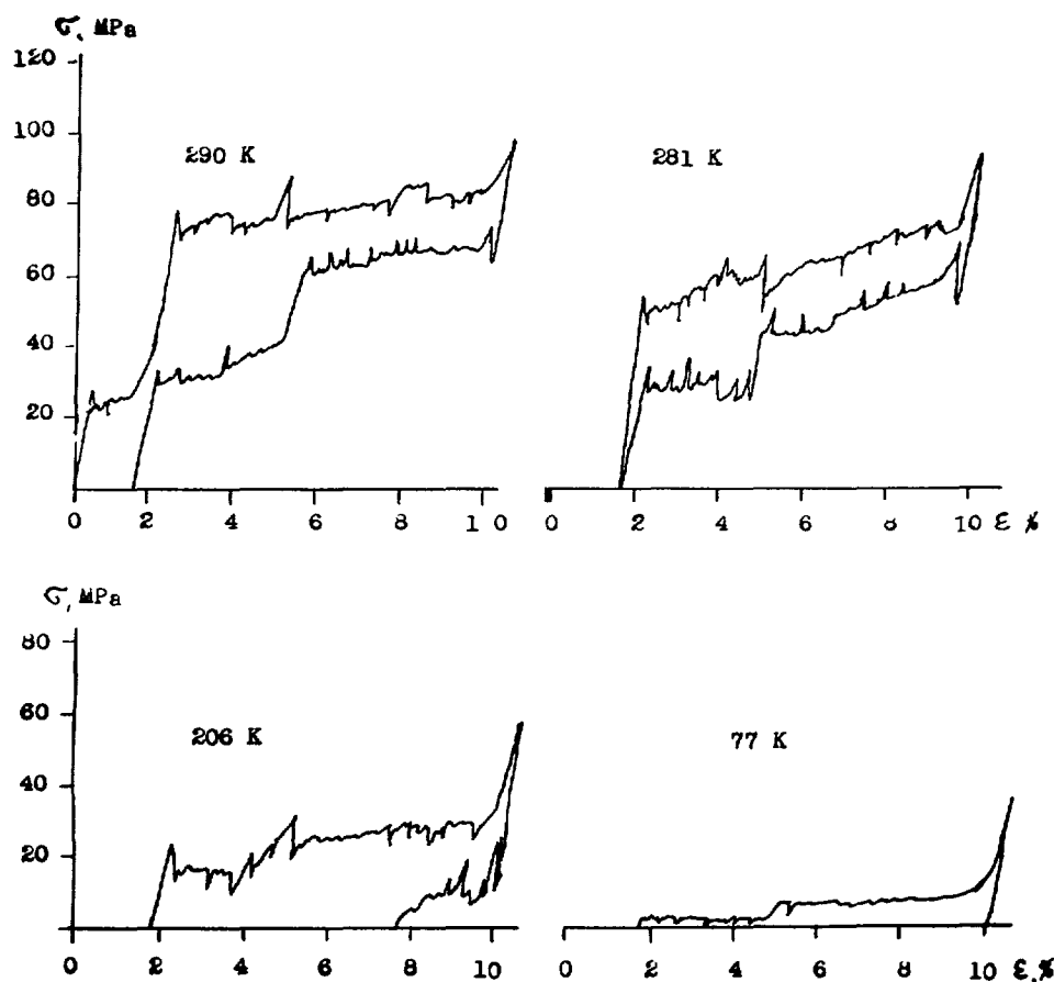
Fig. 7. — Stress-strain curves for tension along the \langle 100 \rangle \beta_1 axis.
