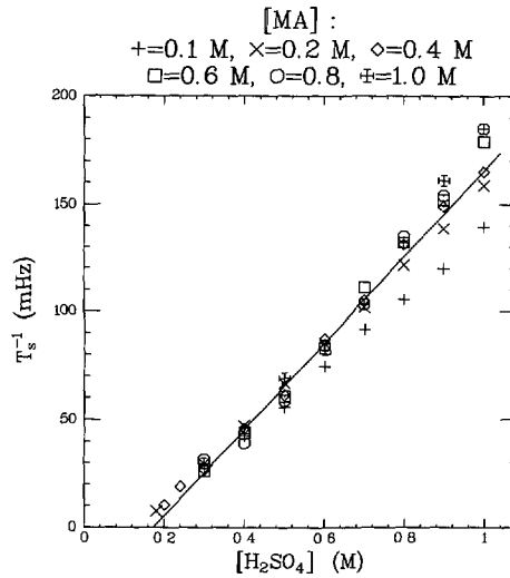
Fig. 12. — The inverse of the spiral period T_s^{-1} vs. [\text{H}_2\text{SO}_4] for several different [\text{MA}] , at [\text{NaBrO}_3] = 0.15 \text{ M} (Fig. 4d).
