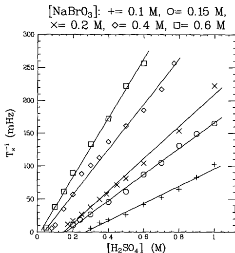
Fig. 10. — The inverse of the spiral period T_s^{-1} vs. [H_2SO_4] for several different bromate concentrations at [MA] = 0.4 M (Fig. 4b).
