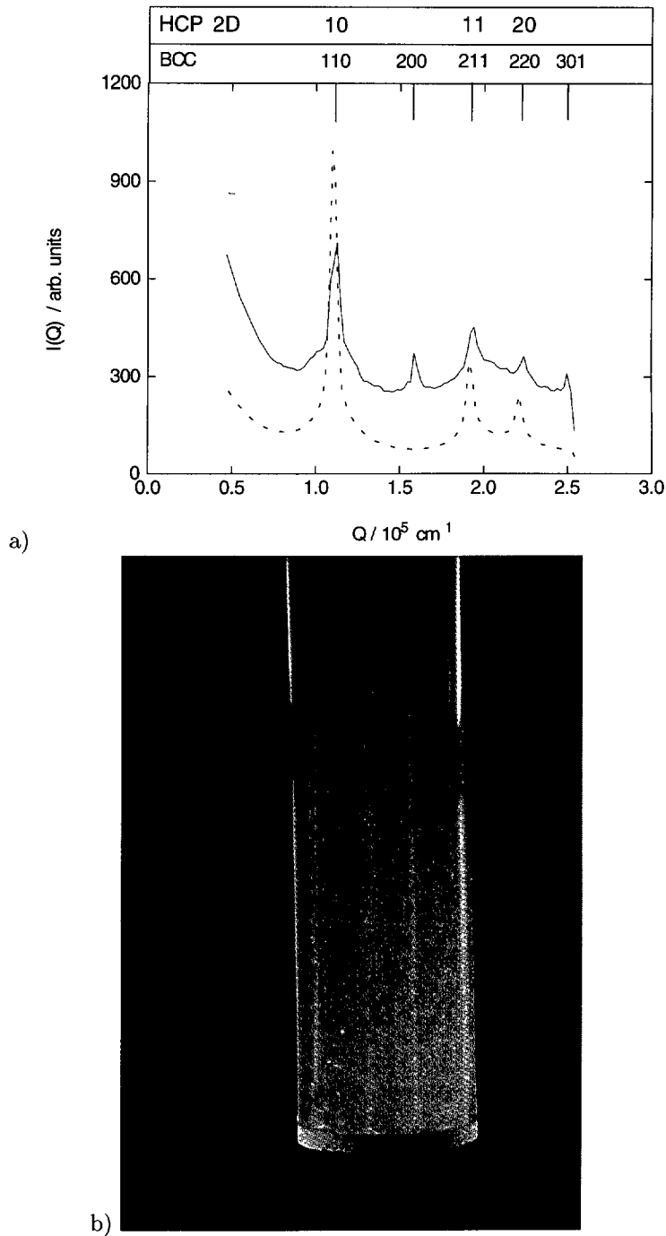
Fig. 6. — a) Light scattering curve ( \lambda = 632.8 \text{ nm} ) of a sample with a volume fraction 0.2%. The solid line corresponds to the scattering of the sample containing crystallites in the bottom of the cell (bcc structure). The dashed line represents the scattering of perceptibly layers in the upper part of the cell. b) Photography of a diluted colloidal crystal. In the lower part, one observes crystallites (bcc structure) while in the upper part layers appear characteristic of non equilibrium structure.
