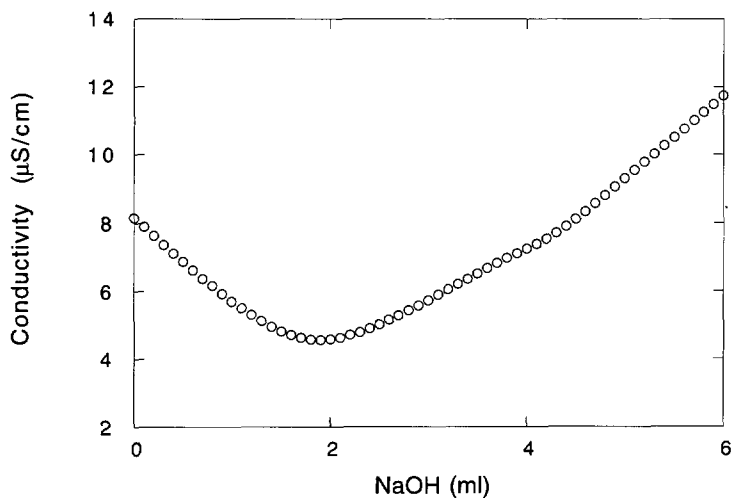
Fig. 3. — Conductimetric titration of a diluted latex suspension (0.13% volume fraction) without added salt; measurement of the conductivity of the solution in \mu\text{S}/\text{cm} versus added 10^{-3} M NaOH.
