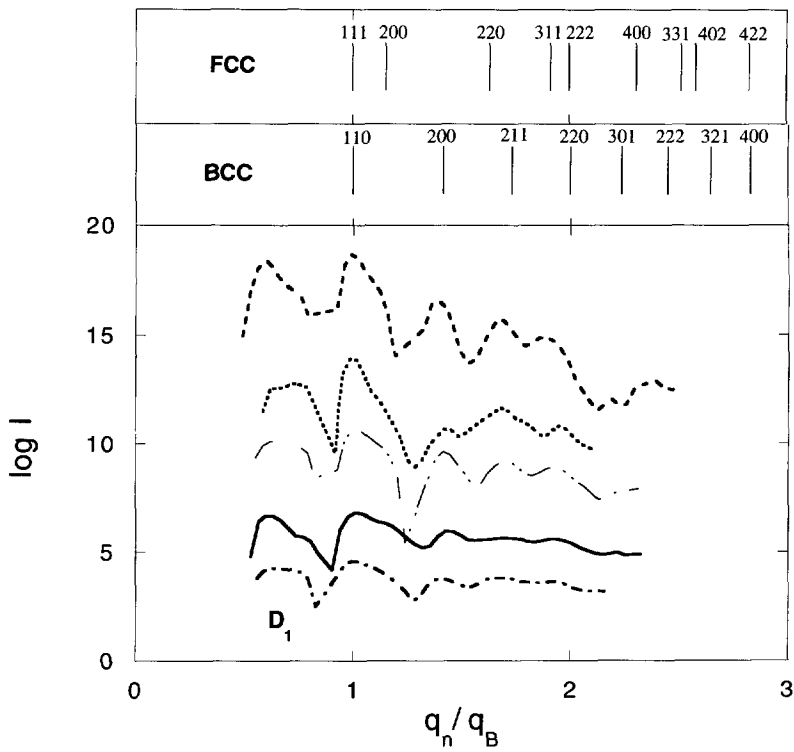
Fig. 9. — Small angle X-ray scattering (USAXS) curves for different volume fractions 2% (---), 3.5% (----), 5.5% (- - - -), 6.5% (- · - ·) and 8% (—) are represented in reduced units q_n/q_B . Peak positions corresponding to a crystal with defects are indicated.
