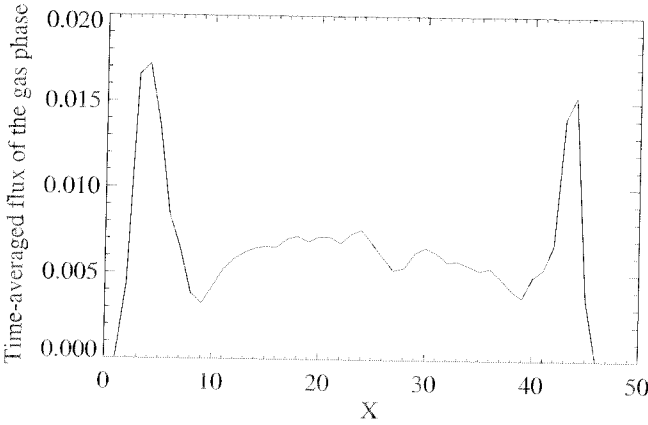
Fig. 7. — Flux of the particles in the gas region, averaged in time and for 16 \leq z \leq 32 for Model A. Notice the important flux in the wetting layers on the side of the channel. In lattice units, the flux is the number of particles per time step.
