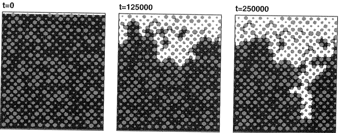
Fig. 9. — Evaporation on a 480 \times 480 lattice with Model A, g_w = 2 and hexagonal grains.
