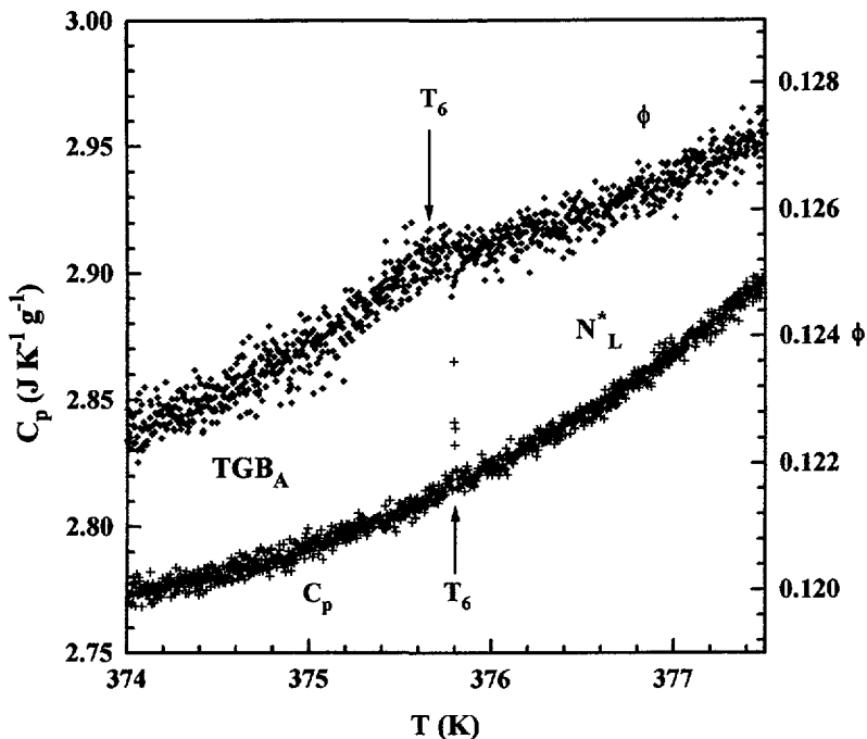
Fig. 4. — Heat capacity C_p and phase shift \phi near T_6 , the TGB A – N_L^* transition temperature, for 10F_2BTFO_1M_7 . These ac mode C_p data were obtained on heating at a scan rate of 50 mK/h, and the \phi data are from a cooling scan at –50 mK/h.
