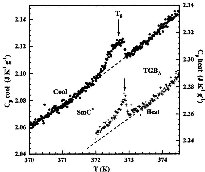
Fig. 5. — Heat capacity measured with the ac mode near T_8 , the \text{SmC}^* - \text{TGB}_A transition temperature, for 10\text{F}_2\text{BTFO}_1\text{M}_7 . Scan rates were \pm 200 mK/h.
