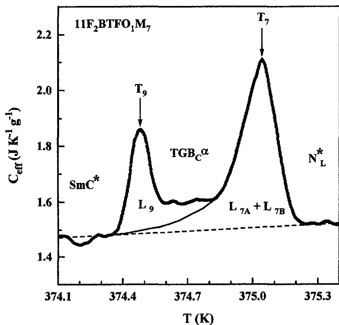
Fig. 8. — C_{\text{eff}}(T) data for 11\text{F}_2\text{BTFO}_1\text{M}_7 obtained with the nonadiabatic scanning technique at a scan rate of +3.5 K/h. The dashed line represents C_p(\text{coex}) ; see the text. The area under the peak labelled T_7 is 143 mJ/g and corresponds to the sum of latent heats L_{7A} + L_{7B} , and the area of 52 mJ/g under peak T_9 represents the latent heat L_9 .
