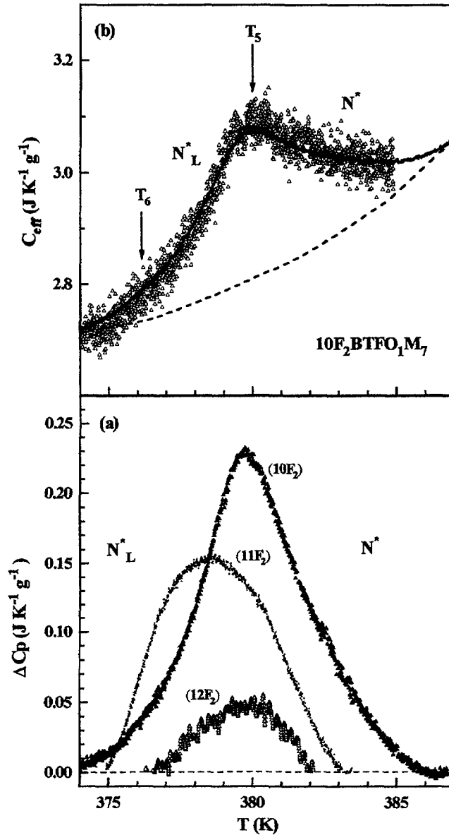
Fig. 2. — (a) Excess heat capacity \Delta C_p = C_p - C_p(\text{background}) for nF_2BTFO_1M_7 obtained from the ac calorimetric data in Figure 1. N_L^* and N^* are not distinct phases but represent a cholesteric with and without short-range twisted line liquid structure. (b) C_{eff}(T) data for 10F_2BTFO_1M_7 obtained with the nonadiabatic scanning technique. The smooth curve represents C_p(ac) data from Figure 1, and the dashed curve is C_p(\text{background}) .
