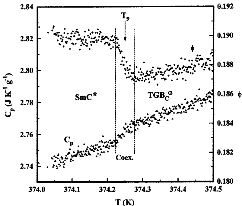
Fig. 10. — Heat capacity and phase shift \phi for 11F_2BTFO_1M_7 in the SmC^* to TGB_C transition region. These ac calorimetric data were obtained on heating at a scan rate of 22 mK/h.
