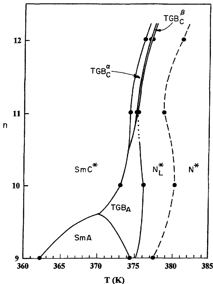
Fig. 12. — Proposed phase diagram for nF_2BTFO_1M_7 based on transition temperatures for n = 10, 11 and 12 determined in the present work and corrected DSC data [12] for n = 9 . The dashed line does not indicate a transition but merely the locus of a C_p maximum in the twisted nematic range.
