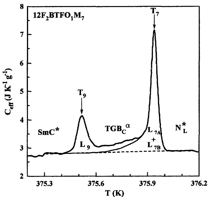
Fig. 9. — C_{\text{eff}}(T) data for 12\text{F}_2\text{BTFO}_1\text{M}_7 obtained with the nonadiabatic scanning technique at a scan rate of +3.5 K/h. The T_7 area is 297 mJ/g and corresponds to the sum of latent heats L_{7A} + L_{7B} , and the T_9 area representing L_9 is 126 mJ/g.
