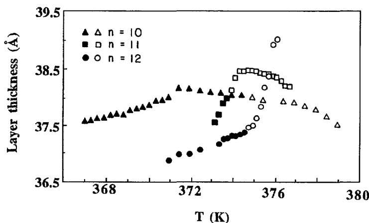
Fig. 3. — Layer spacing d as obtained from an X-ray study of nF 2 BTFO 1 M 7 [10]. The open symbols were obtained from diffuse diffraction peaks, indicating only short-range order, and the solid symbols were obtained from sharp resolution-limited ( 6.2 \times 10^{-4} \text{ \AA}^{-1} ) peaks.
