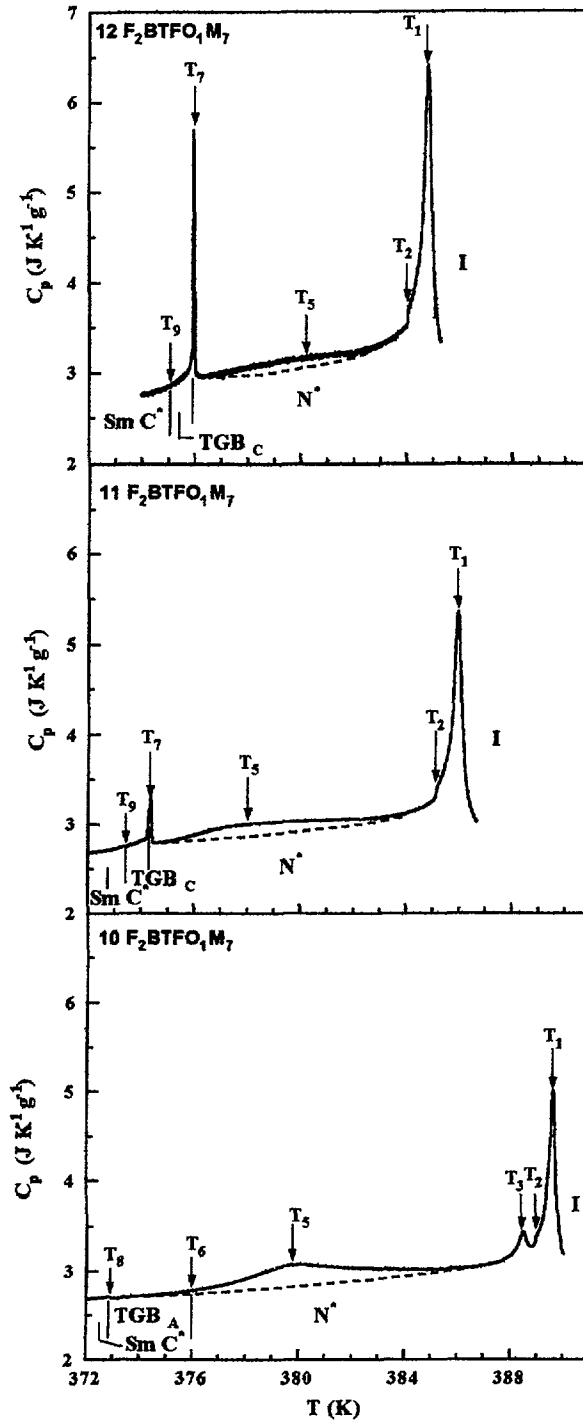
Fig. 1. — Heat capacity of three n\text{F}_2\text{BTFO}_1\text{M}_7 compounds measured with the ac calorimetric mode. The dashed line represents C_p (background), the behavior expected in the N^* phase in the absence of short-range TGB ordering.
