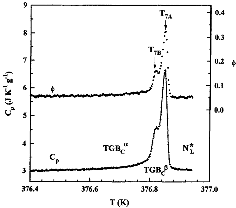
Fig. 7. — Heat capacity and phase shift \phi for 12F_2BTFO_1M_7 in the N_L^* to TGB C transition region. These ac calorimetric data were obtained on cooling at a scan rate of -30 mK/h.
