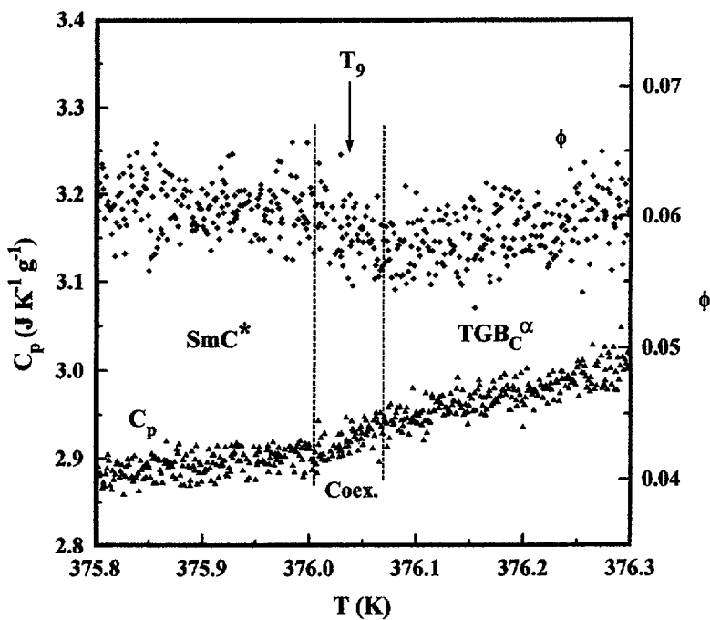
Fig. 11. — Heat capacity and phase shift \phi for 12F_2BTFO_1M_7 in the SmC^* to TGB_C transition region. These ac calorimetric data were obtained on heating at a scan rate of 15 mK/h.
