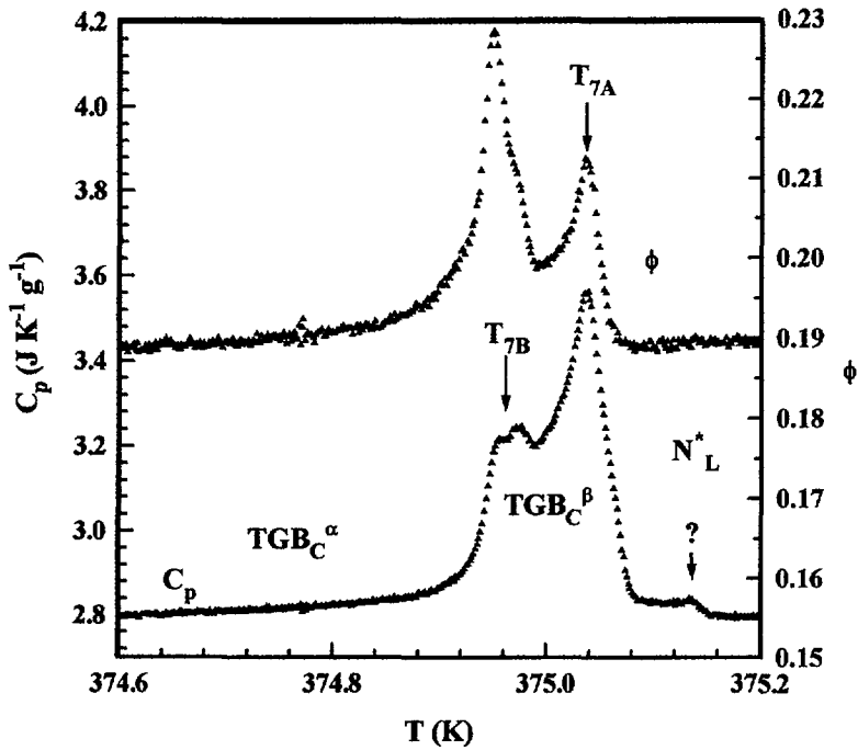
Fig. 6. — Heat capacity and phase shift \phi for 11F_2BTFO_1M_7 in the N_L^* to TGB C transition region. These ac calorimetric data were obtained on heating at a scan rate of 22 mK/h.
