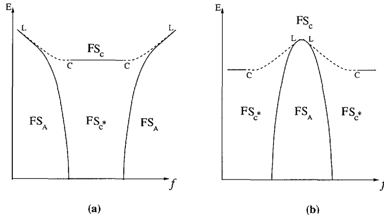
Fig. 11. — A possible schematic phase diagram of a \epsilon_a > 0 ferrosmectic in crossed fields. For (a) \alpha > 0 , \chi_a > 0 and \mathbf{M} \cdot \mathbf{H} < 0 . (b) \alpha < 0 , \chi_a < 0 and \mathbf{M} \cdot \mathbf{H} > 0 . The full line represents second order phase transition and the dashed line the first order transition. Points C and L represent tricritical and Lifshitz points. Here f = (\chi_a H^2 + MH) .
