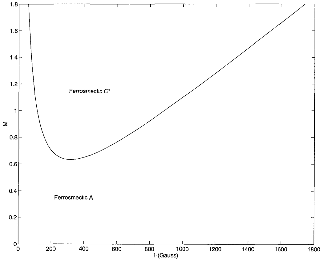
Fig. 3. — The phase diagram for the achiral FS A phase. Here \alpha = 1 , \beta = 0.1 , \chi_a = 0.1 \times 10^{-6} and \mathbf{M}_z and \mathbf{H} are anti-parallel to one another. \mathbf{M} is in units of 10^4 Gauss.
