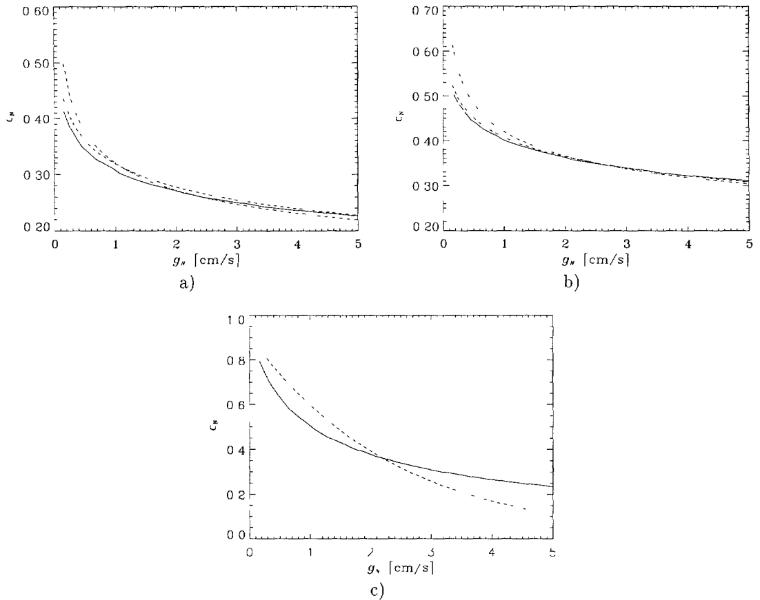
Fig 2 — a) Restitution coefficient \epsilon_N vs. impact velocity g_N - comparison of our model with the experiments made with frost covered spheres [2] Dash-dotted experimentally obtained curve Dashes curve obtained using equation (30). Solid line curve obtained using equation (25) b) Restitution coefficient \epsilon_N vs. impact velocity g_N - comparison of our model with the experiments made with frost covered spheres [3] Dash-dotted experimentally obtained curve Dashes curve obtained using equation (30) Solid line curve obtained using equation (25) c) Restitution coefficient \epsilon_N vs. impact velocity g_N - comparison of Poschl's model with the experiments performed with clean, smooth spheres [3] Dashed experimentally obtained curve Solid line Poschl's model with A_2 = 0.75
