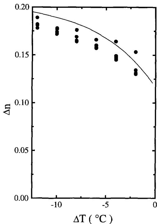
Fig. 12. — Birefringence \Delta n of 5CB versus \Delta T = T - T_{Iso} . The solid line displays the data communicated by BDH-Merck
