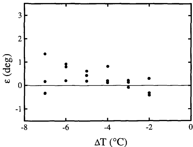
Fig 13 — Pretilt angle \epsilon of 7BPI in the SmA phase obtained on the PTFE treated surfaces versus \Delta T = T - T_{Iso} , for different places in the sample.
