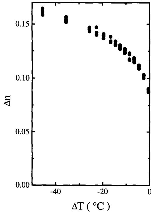
Fig. 10. — Birefringence \Delta n of 20O6 versus \Delta T = T - T_{\text{Iso}}
