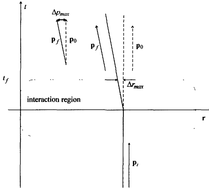
Fig. 1. — Perturbed (solid line) versus unperturbed (dashed line) atomic trajectories. At time t = t_f where the atoms exit the interaction region with the diffraction grating, the maximum deviation in momentum (resp. in position) between the perturbed and unperturbed atomic trajectories is \Delta p_{max} (resp. \Delta r_{max} ).
