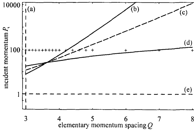
Fig. 2. — Regions of validity of the semiclassical approach, as a function of Q and P_1 = p_1/\hbar\kappa . The modulation depth was taken as \epsilon = 1 . The semiclassical approach is valid in the region between the lines (b) and (d). The line (c) ( u = 1 ) separates the regimes of high (above) and low (below) modulation index u . (a) Line Q = 3 , (Eq. (4.30)) defining the region for a fast classical micromotion of the atom. (b) Limit 2(\Delta P_{\text{max}})^2 = P_1 , (Eq. (4.39)). (d) Limit 2Q^2 = P_1 , (Eq. (4.38)). (e) Limiting condition p_1 = \hbar\kappa for the semiclassical regime. Crosses: parameters corresponding to the numerical solution (Fig. 1 and Sect. 5).
