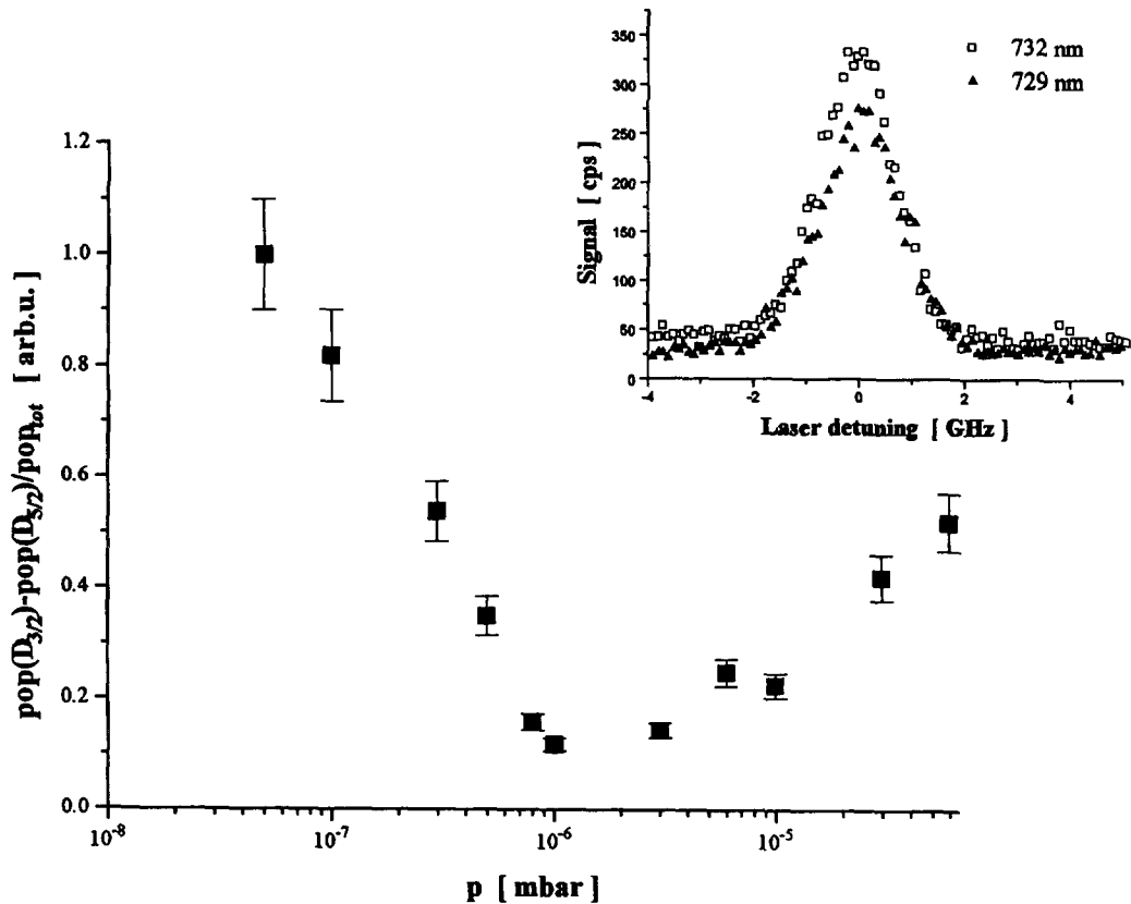
Fig. 10. — Population difference of the 3D_{5/2} and 3D_{3/2} levels as a function of buffer gas pressure. At 10^{-6} mbar, the levels are almost completely mixed. Inset : fluorescence intensities of both forbidden transitions, although only the D_{3/2} -state is directly populated at 2 \times 10^{-6} mbar.
