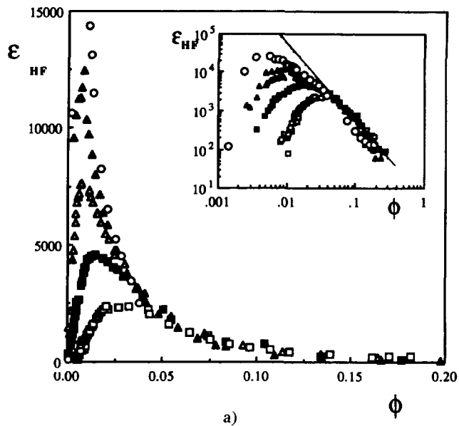
Fig. 19. — (a) Intensity of the high frequency mode for samples with different salt concentrations as a function of the membrane volume fraction. The same data are given in inset with a log-log scale to emphasize the scaling law \epsilon_{hf} \sim 1/\phi^2 obtained above \phi^* (b) Characteristic frequency of these samples. Same symbols as before.
