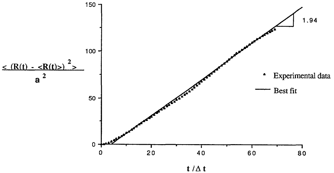
Fig. 4. — Mean-square displacement \sigma^2(t) = \langle (\mathbf{R}(t) - \langle \mathbf{R}(t) \rangle)^2 \rangle of the particles as a function of time in the experimental case of figure 3. \sigma^2 is rendered dimensionless by the square of particle diameter a^2 , and the time t by the time step \Delta t used for the acquisition of the successive positions of the particles (here \Delta t = 6 s).
