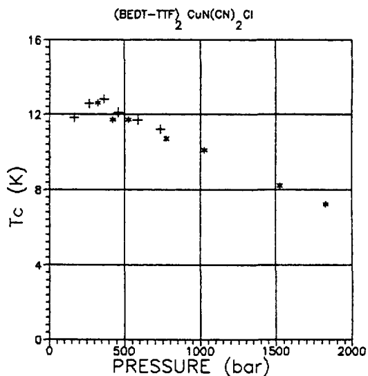
Fig 3 — Pressure dependence of superconducting transition temperature of \kappa -(BEDT-TTF) _2 CuN(CN) _2 Cl samples. Symbols (+) denote resistivity midpoint values we reported, symbols (*) represent the data reported by Williams et al. [1].
