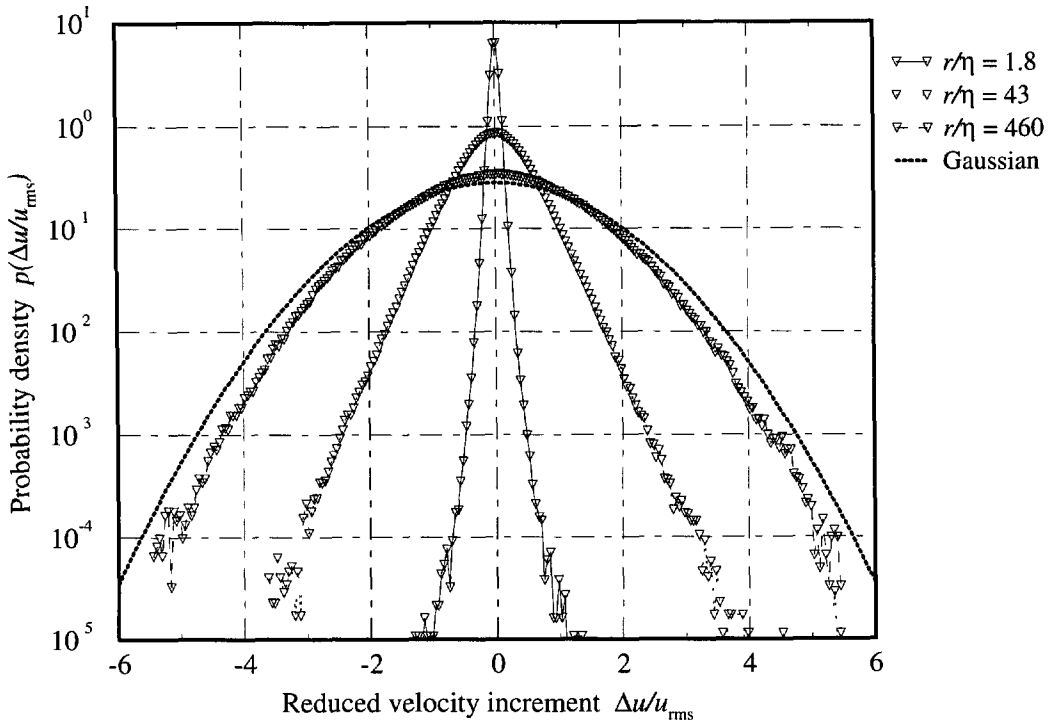
Fig. 1. — pdf of transverse velocity increments reduced by the rms velocity at various separations in units of the Kolmogorov dissipation scale \eta . (From Ref. [46].)
