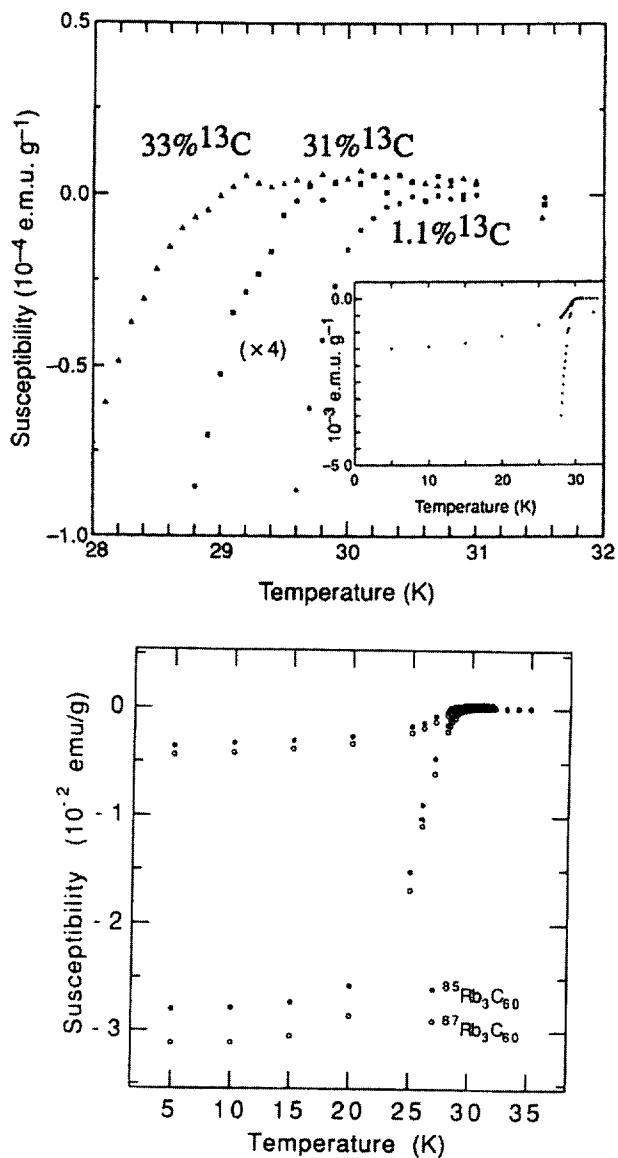
Fig. 7. — Isotope effects of ^{13}\text{C} and ^{87}\text{Rb} on superconducting transition temperature in \text{Rb}_3\text{C}_{60} .
