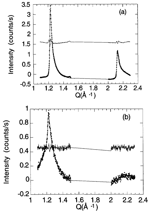
Fig. 3. — 0.85 \text{CCl}_4 monolayer diffraction profiles at 40 K (a) and at 197 K (b). Solid lines are double Lorentzian fits for each peak and difference between observed and calculated intensity.
