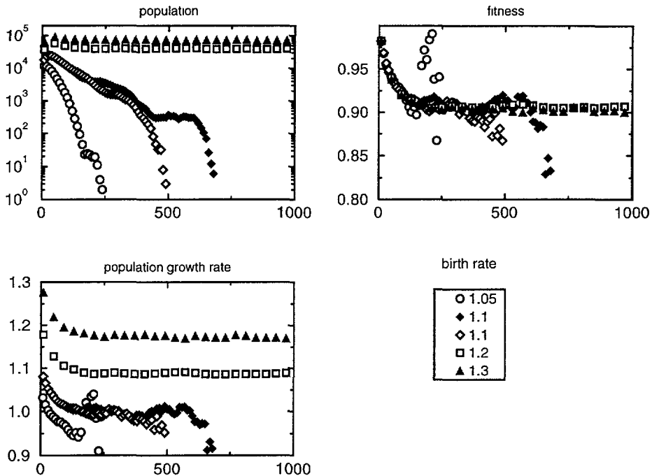
Fig. 5. — Time evolution of the population (on top-left), population mean fitness (on top-right) and population growth rate r for outcrossing S = 0 populations under multiplicative selection obtained for different birth rates (presented in the legend). For birth rate Birth = 1.2 and 1.3 the population stabilizes around different values, as well as the population growth rate and instead of it the fitness stabilizes around the same value. For Birth = 1.05 and 1.1 we observe the mutational meltdown of these species. For all simulation we start with N(0) = 10,000 . For Birth = 1.1 we performed two different simulations using different seeds for the random number generator, in order to avoid mistakes due statistical fluctuations. One can observe the fluctuation of the fitness around the characteristic value of this set of parameters for Birth = 1.1 before extinction (black diamonds). In text are mentioned the value of the distinct parameters.
