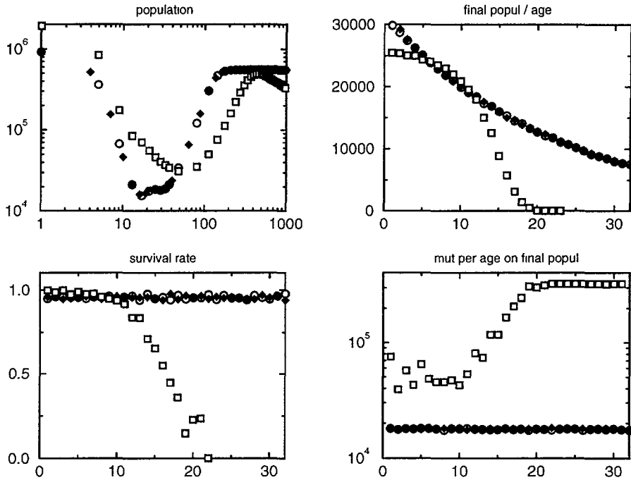
Fig. 8. — Penna model: temporal evolution of the population (on top-left), age-distribution of population (top-right), survival rate (bottom-left) and distribution of deleterious mutations in final populations for m = 1 , limit = 3 , birthr = 0.2 , min\_age = 8 and initial populations 2 \times 10^6 . The final populations stabilizes (not showed for asexual reproduction). Black diamonds and white circles represent sexual individuals (males and females, respectively). White squares represent asexual population. Note that the survival rate for sexual populations remains constant (for discussion see text).
