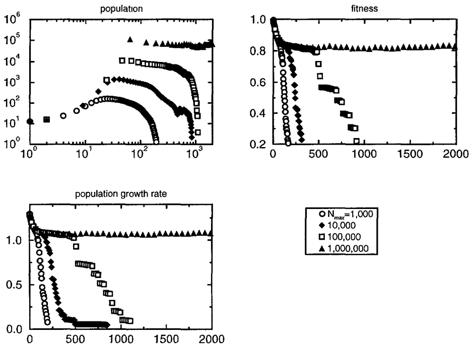
Fig. 7. — Time evolution of the population (on top-left), population mean fitness (on top-right) and the population growth rate (bottom/left) for outcrossing S = 0 populations under multiplicative selection obtained for initial population N(0) = 10 with different N_{max} (shown in the legend). The collapse of the species can be avoided by a enough growth, that means, diversification.
