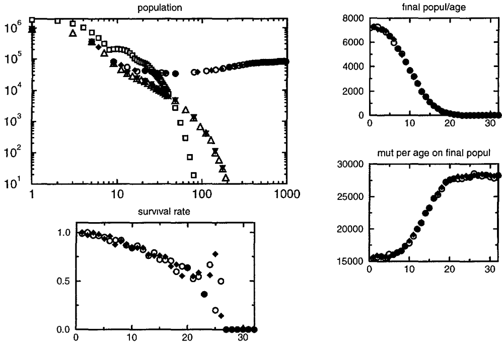
Fig. 9. — Penna model: temporal evolution of the population (on top-left), age-distribution of population (top-right), survival rate (bottom-left) and distribution of deleterious mutations in final populations with m = 8 , limit = 3 , min\_age = 8 and initial populations 2 \times 10^6 for different birth rate. Black and white triangles (males and females, respectively) represent sexual population with birth_r = 0.4 . Due to the accumulation of harmful mutations the population becomes extinct. By changing the birth rate to 0.7 (black diamonds and white circles) we can avoid the extinction of the species and the populations stabilizes. Now the survival rate decays with age and we can observe an accumulation of harmful mutations in old ages. The asexual population does not survive with the same parameters (white squares).
