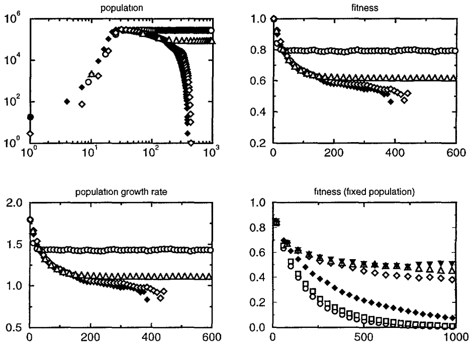
Fig. 6. — Time evolution of the population (on top-left), population mean fitness (on top-right) and the population growth rate (bottom/left) for selfing S = 1 or outcrossing S = 0 populations under multiplicative selection obtained for initial population N(0) = 10 and N(0) = 2 (white diamonds) and different recombination rate recl (described in text). We used here mutr = 0.5 , Birth = 1.8 and the Verhulst parameter N_{max} = 1,000,000 , the selection coefficient and the dominance coefficient have the same value cited above. The bottom/right plot shows the time evolution of the fitness for fixed population (from bottom to top in the figure the symbols represent population sizes N = 50, 100, 500, 5,000, 10,000 and 20,000 , averaged over 20 samples).
