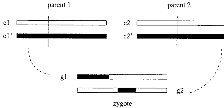
Fig. 1. — Schematic representation of the mating process. Parent is a diploid cell with two paired (homologous) chromosomes. A recombination event generates the gamete g1 . Similarly, the gamete g2 is generated from the parent 2 . The fusion of these two gametes results in the zygote . For details and description see text.
