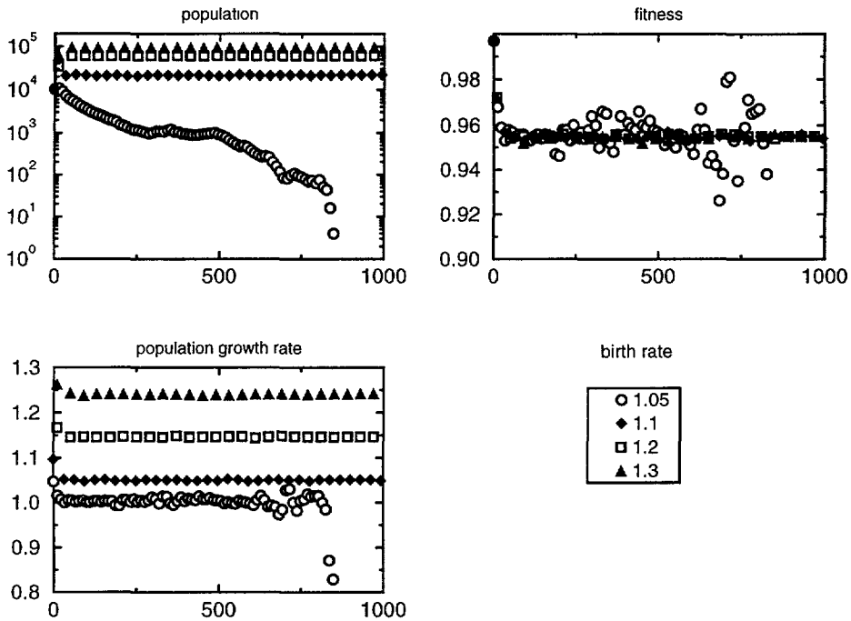
Fig. 4. — Time evolution of the population (on top-left), population mean fitness (on top-right) and fitness times birth rate (the population growth rate r ) for selfing S = 1 populations under multiplicative selection obtained for different birth rates (presented in the legend). For birth rate Birth = 1.1, 1.2 and 1.3 the population stabilizes around different values, as well as the population growth rate and instead of it the fitness stabilizes around the same value. For Birth = 1.05 we observe the mutational meltdown of these species. For all simulation we start with N(0) = 10,000 . In text are mentioned the value of the distinct parameters.
