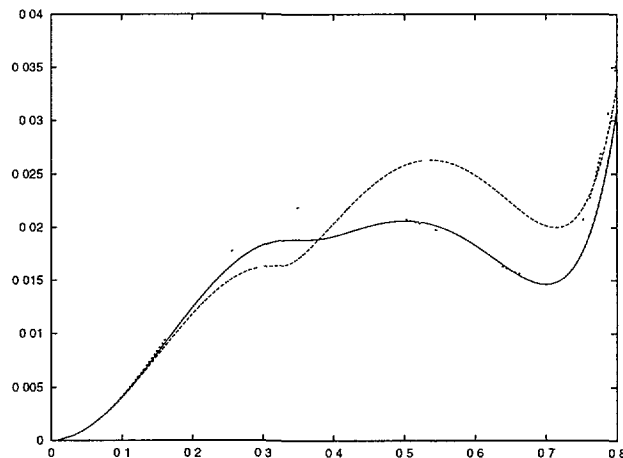
Fig. 3. — The potential for f(q) = 1/2(q^3 + q^4) for \beta' = (\beta_D + \beta_s)/2 = 1.27 and \beta = 1.21 (dots) \beta = 1.31 (full line) and \beta = 1.41 (dashes).
