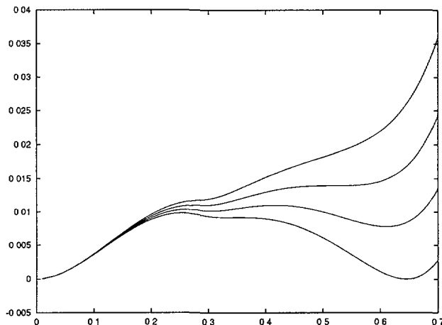
Fig. 2. — The potential for the p = 3 -spin model and different temperature. The curves are drawn for \beta = \beta_s and, from top to bottom, \beta' = 1.59, \beta' = \beta_D = 1.63, \beta' = 1.66, \beta' = \beta_S = 1.70 .
