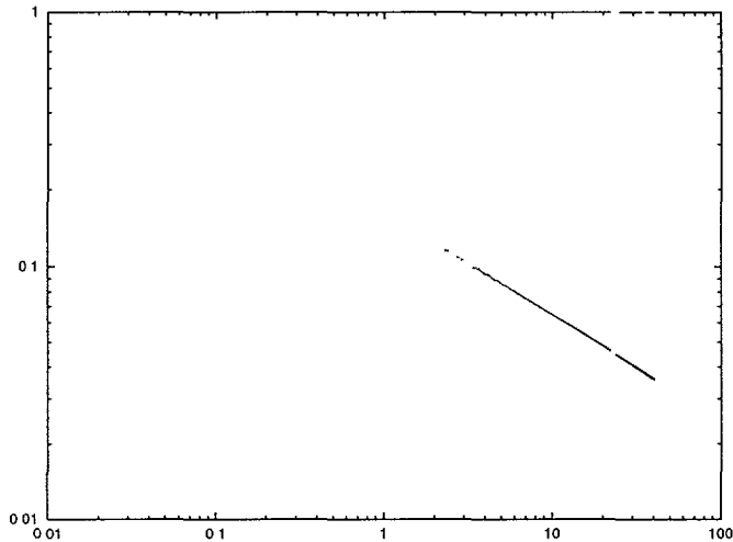
Fig. 4. — The convergence of C(t, 0) to \tilde{p} for the 3+4 model in the case T = 0.673 , T' = 0.804 . We plot C(t, 0) - \tilde{p} as a function of t in a log-log scale, for \tilde{p} we take the value in the primary minimum of the potential \tilde{p} = .646 . C(t, 0) - \tilde{p} seems to approach zero as a power law. A similar plot is found for the energy as a function of time.
