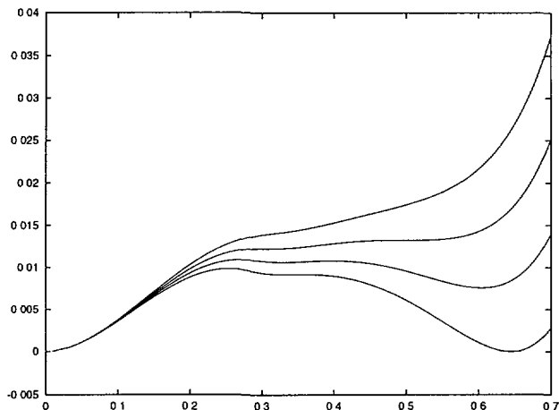
Fig. 1. — The potential function in the p = 3 -spin model for T = T' and various temperatures. From top to bottom \beta = 1.59, \beta = \beta_D = 1.63, \beta = 1.66, \beta = \beta_S = 1.70 . Observe that a minimum is first present at the dynamic temperature and the value of the minimum of potential at the statical temperature is zero.
