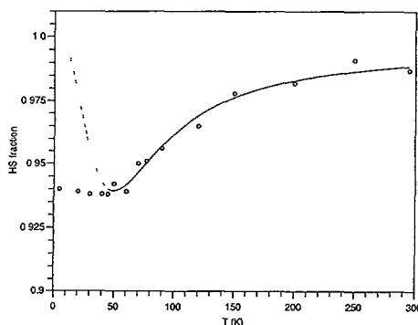
Fig. 10. — Experimental conversion curve of \text{Fe}^{\text{II}}(\text{TRIM})_2\text{F}_2 , where TRIM = 4 1 -(4-methylimidazole) [14], with the best-fit curve using the present electron-vibrational model. The low temperature branch of the computed (equilibrium) curve is not experimentally reached because of the slow kinetics of the spin conversion; it was given a null statistic weight for the fit. The parameter values which fit the equilibrium branch data ( T \geq 50 K) are \Delta_0 = 356 K, \omega_{\text{LS}} = 232 K, \omega_{\text{LS}}/\omega_{\text{HS}} = 1.30 . The electro-vibrational ground state is HS; the first excited level is a low-lying ( \sim 43 K) LS state.
