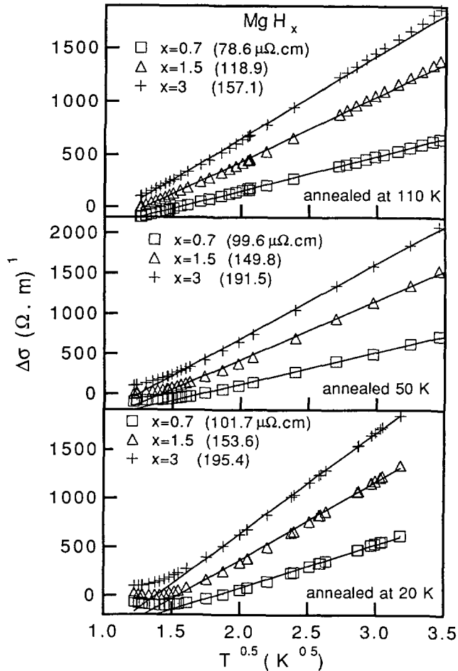
Fig. 7. — Conductivity temperature dependence for three different films ( x = 0.7, 1.5 and 3 ) annealed at 20\text{ K}, 50\text{ K} and 110\text{ K} . For the first two anneals, the conductivity begins to increase at T \leq 2\text{ K} . This is related to the non-percolating superconducting phase discussed in the text. (The curves have been shifted vertically).
