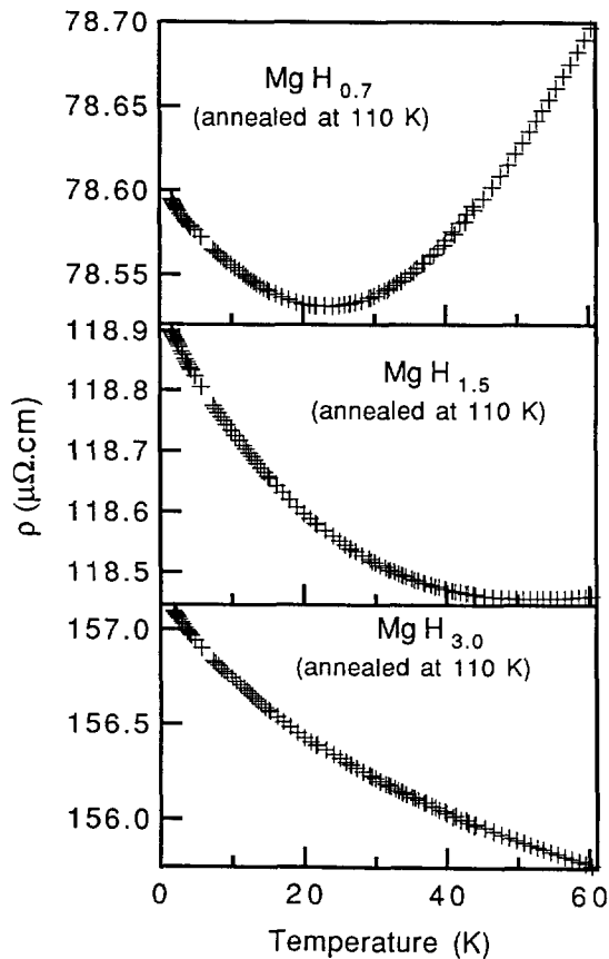
Fig. 6. — Resistivity temperature dependence of the high concentration films annealed at 110 K ( x = 0.7, 1.5 and 3 ).
