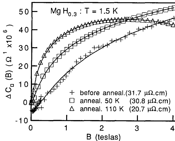
Fig. 5. — Magnetoconductance curves of an \text{MgH}_{0.3} film for different annealing temperatures. The solid lines are calculated with the weak localization and Kohler contributions. Note the negative magnetoconductance for the non annealed film.
