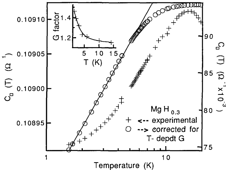
Fig. 4. — The experimental variation (+) of the conductance can be transformed into a 2D logarithmic variation (o) with temperature by taking into account the coefficient G related to the inhomogeneity. G is deduced from the magnetoconductance analysis.
