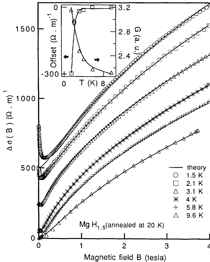
Fig. 8. — Negative and positive magnetoconductance for \text{MgH}_{1.5} at different temperatures. For clarity the curves have been offset relative to each other. The vertical scale corresponds to the lowest curve. The solid lines correspond to the positive 3D weak electron localization (Eq. (6)) and the resulting values for G and the offset are shown in the inset.
