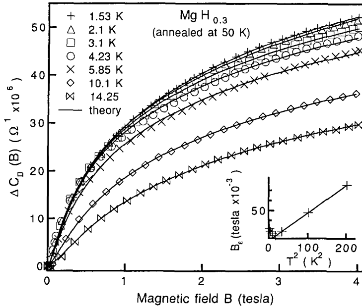
Fig. 3. — Positive magnetoconductance of a MgH 0.3 film at different temperatures. The solid lines are the fits to equation (3). The deduced inelastic magnetic field B_e are shown in the inset.
