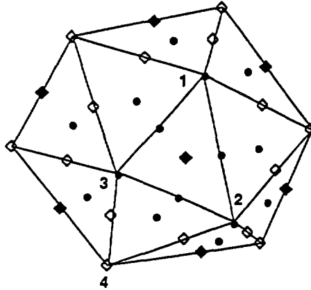
Fig. 2. — The set of the most important strong (◆), weak (●) and planar (◇) periodic directions in the rhombohedral approximant. These periodic directions are shown relatively to the axes of the icosahedral quasicrystal.
