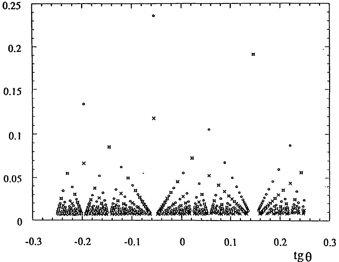
Fig. 1. — The plot of the inverse of the period 1/P vs. the slope \text{tg } \theta for the hyperlattice vectors belonging to the HTP corresponding to a fivefold axis (O) and to a [\tau, 1, 0] type axis (x) in a P-type hyperlattice (the hypercube edge length is unity).
