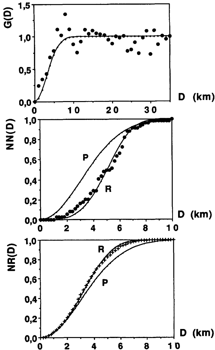
Fig. 10. — The pair correlation function g(D) , the distributions NN(D) and NR(D) measured for Spanish towns (full circles and crosses, Sect. 2.2, [22, 23]). Bold lines are calculated from equations (13) ( g(D) ), (12) ( R ), (10) ( R ) respectively for \sigma = 4.372 km (Rel. (9)). The bold lines marked P are calculated for a Poisson point process ( NN(D) = NR(D) = 1 - \exp(-D^2/\sigma^2) ).
