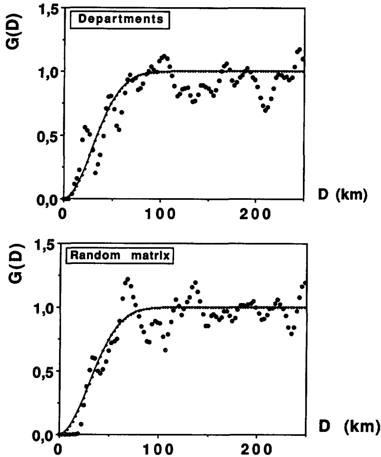
Fig. 11. — The pair correlation function for chief towns of departments ( N = 64 ) in W (Fig. 13) and for N = 66 eigenvalues of an asymmetric complex random matrix taken in a rectangle W' ( W and W' are homothetic). Bold lines are calculated using relations (9) and (13).
