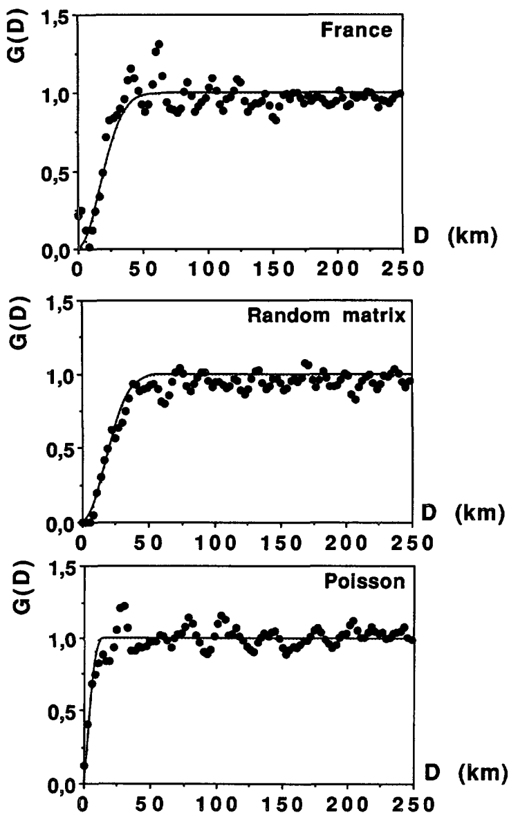
Fig. 14. — Pair correlation functions g(D) for the point processes of figure 13 (bold lines : Rel. (13), \sigma is calculated from Rel. (9) except for the Poisson point process).
