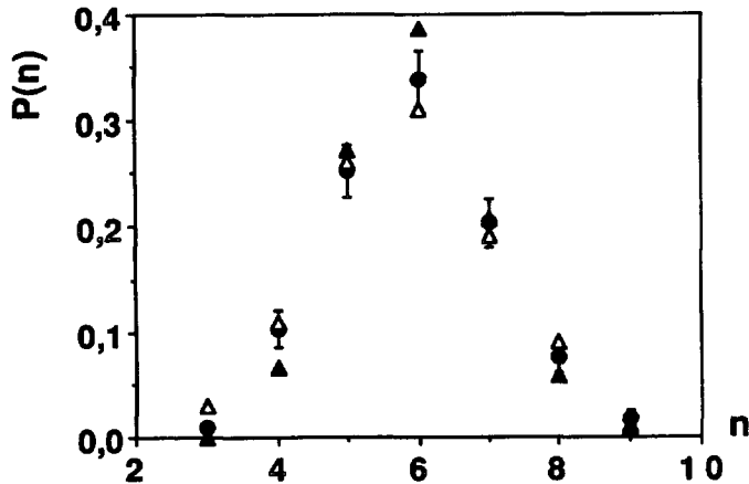
Fig. 3. — Distribution P(n) of the number of edges for NF districts (full circles with error bars, \mu_2 = 1.41 ), for 2D cellular arrays formed during the directional solidification of Pb-30 wt% Tl alloys with a growth velocity V = 0.75 cm/h (empty triangles, \mu_2 = 1.58 , [6]) and for an undifferentiated vegetable tissue of Anthurium ( N = 1\,295 , full triangles, \mu_2 = 1.10 , [32]).
