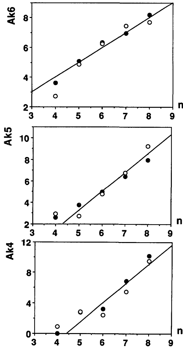
Fig. 5. — Correlations A_{kn} ( 4 \leq n, k \leq 8 ) for NF districts (full circles, \mu_2 = 1.41 ) and for a tissue of Anthurium (open circles, \mu_2 = 1.10 , Mombach et al. , [32, 35]) (straight lines: Eq. (5) with a/\mu_2 = 0.755 ).
