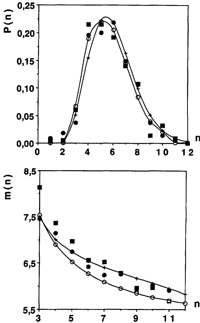
Fig. 7. — Distributions P(n) and correlations m(n) for Devon and Somerset (full squares, \mu_2 = 4.62 , and full circles, \mu_2 = 3.62 , respectively, Boots, 1980, [10]), for an iron polycrystal isothermally annealed at 650 °C during 125 min (open circles and bold line, \mu_2 = 3.59 , m(n) is given by 5 + 7.6/n , Hu [40]) and for a 12-6-4 topological model (crosses and bold line, \mu_2 = 3.13 , [16]).
