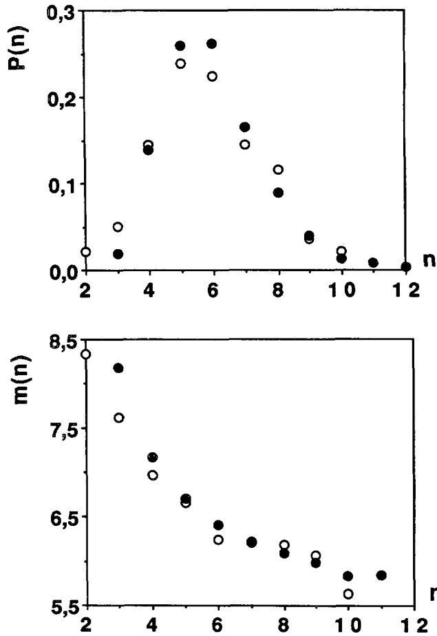
Fig. 6. — Distributions P(n) and correlations m(n) for Wiltshire (open circles, \mu_2 = 2.91 , Boots, 1980, [10]) and for an alumina cut (full circles, \mu_2 = 2.59 , Righetti et al. , [39]).
