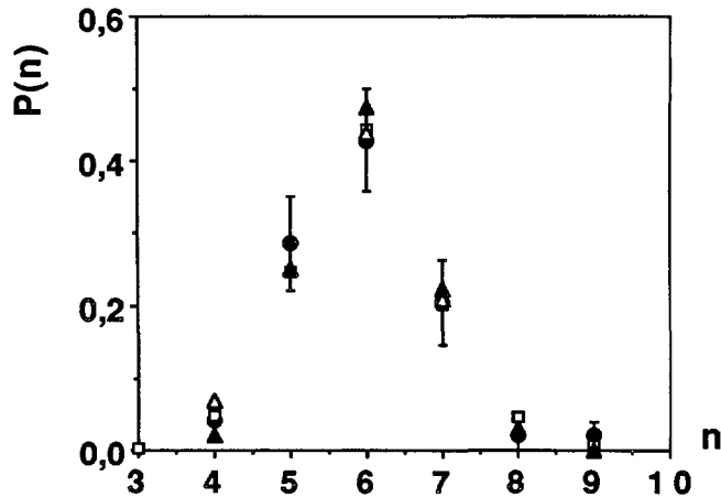
Fig. 2. — Distribution P(n) of number of sides for NF departments (full circles with errors bars, \mu_2 = 0.91 ), for an epidermal epithelium of a 100 mm cucumber (Tab. I, full triangles, \mu_2 = 0.64 , [3]), for 2D cellular arrays formed during the directional solidification of Pb-30 wt% Tl alloys with a growth velocity V = 0.85 cm/h (empty triangles, \mu_2 = 0.85 , [6]) and for a young soap froth (empty squares, \mu_2 = 0.93 , Delannay, unpublished).
