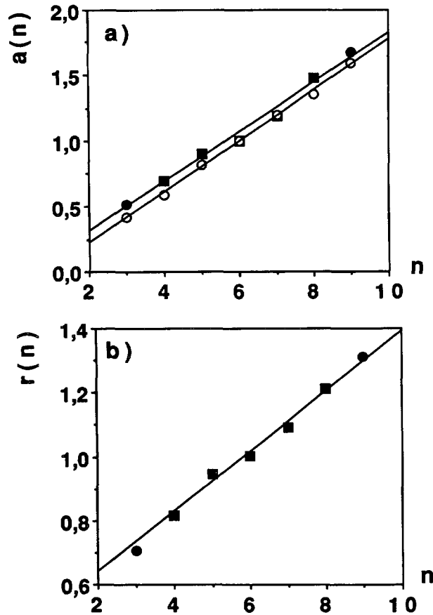
Fig. 8. — a) Average normalized area of n -cells a(n) for NF districts (full squares and full circles) and for human amnion (open circles, Lewis 1928, [3]); b) associated radius r(n) = \{a(n)/\pi\}^{1/2} for NF districts as a function of n .
