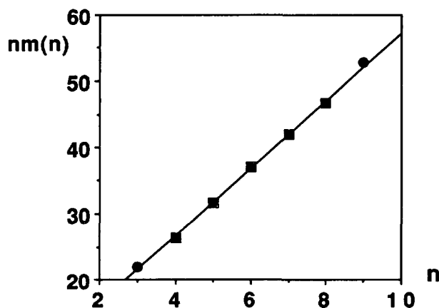
Fig. 4. — Average correlation nm(n) as a function of n for NF districts (Aboav-Weaire line, see Tab. III). The statistical significance of 3m(3) and 9m(9) (full circles) is weak as there are only 2 and 4 districts with 3 and 9 edges respectively.
