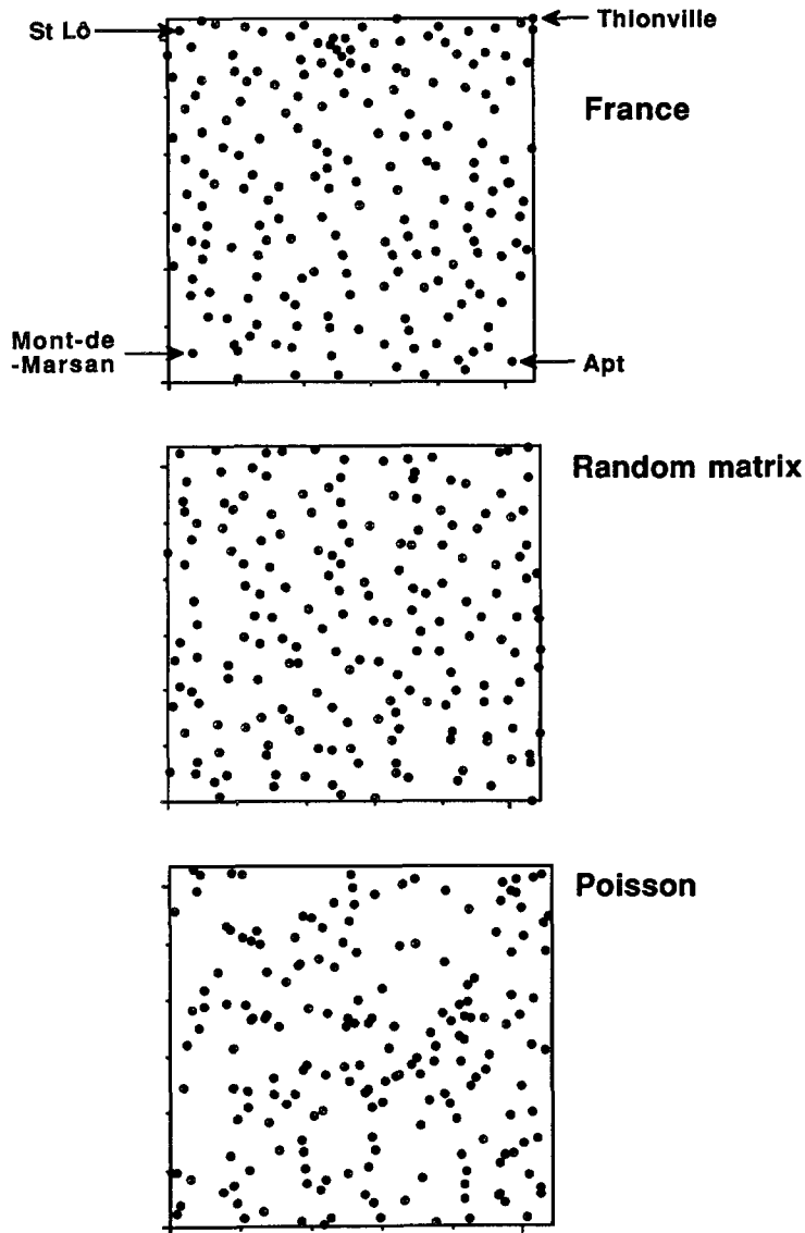
Fig. 13. — 188 chief towns of districts in a rectangle W ( 544 \times 636 km), 184 eigenvalues of a complex 600 \times 600 random matrix in a rectangle W' , 187 points of a Poisson point process in W' ( W and W' are homothetic).
