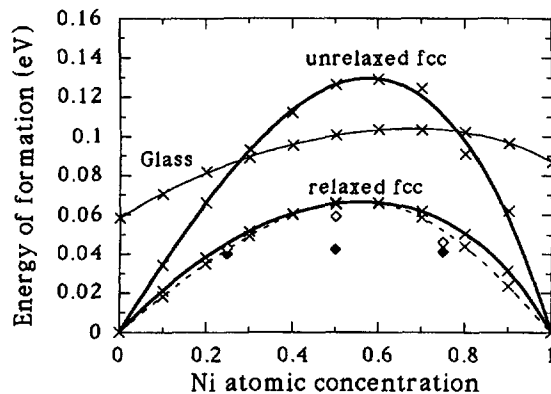
Fig. 2. — Formation energies of the \text{Au}_{1-x}\text{Ni}_x solid solutions and glasses versus Ni concentration. The crosses (x) indicate the results obtained in this work (with 4 000 atoms) : the unrelaxed energy is calculated with Vegard's law lattice parameter, this is the initial state for the relaxation at zero pressure. The dotted line extrapolates at 0 K the experimental results of Hultgren (see text). Three computed metastable compounds are drawn on this figure (white rhombus : initial state ; black rhombus : relaxed state).
