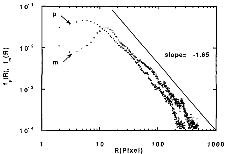
Fig. 14. — Pore and mass chord distribution functions calculated from the digitized image 13. Full squares : the pore (p) ; Open circles : the solid (m).
