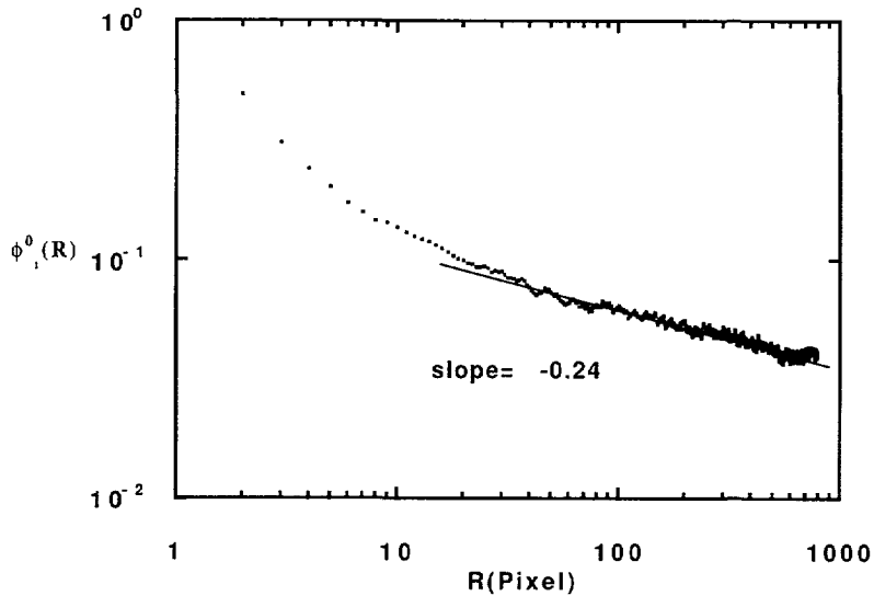
Fig. 16. — « Interfacial » conditional autocorrelation function calculated from the digitized image shown in figure 13 (see text for definition).
