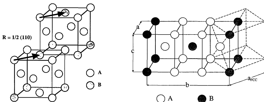
Fig. 1. — a) The DO 22 structure : the arrows show the periodic antiphase displacements along \langle 1/2 \ 12/0 \rangle transforming the L1_2 into the DO 22 structure. b) The Pt 2 Mo-like structure (solid lines) : the dashed lines represent the underlying FCC structure.
