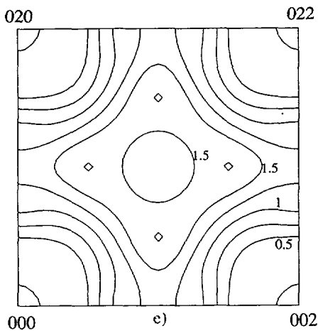
Fig. 6. — a) Short-range order intensities in the (100) plane for \text{Pd}_3\text{V} at 840^\circ\text{C} . Laue units. b) Short-range order intensities in the \langle 100 \rangle plane for \text{Ni}_3\text{V} at 1100^\circ\text{C} . Laue units. c) Short-range order intensities in the \langle 100 \rangle plane for \text{Ni}_2\text{V} at 955^\circ\text{C} . Laue units. d) Short-range order intensities in the \langle 100 \rangle plane for \text{Ni}_3\text{Cr} at 560^\circ\text{C} . Laue units. e) Short-range order intensities in the \langle 100 \rangle plane for \text{Ni}_2\text{Cr} at 650^\circ\text{C} . Laue units.
