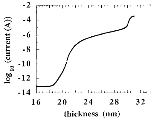
Fig. 1. — Experimental current versus thickness curve obtained at room temperature. Deposition rate: 0.05 \text{ nm.s}^{-1}
