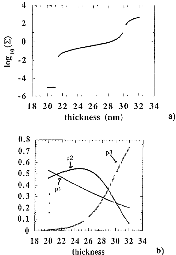
Fig. 2. — a) Conductance versus thickness curve calculated using the EMA approximation. The conductivity before 21 nm has arbitrarily been fixed at 10^{-5} S.cm ^{-1} . The figure 2b shows the evolution of p_1 , p_2 and p_3 . The following values have been assumed in equation (5): \epsilon_1 = 21 , \epsilon_3 = 30 , w_1 = 8 and w_3 = 2 .
