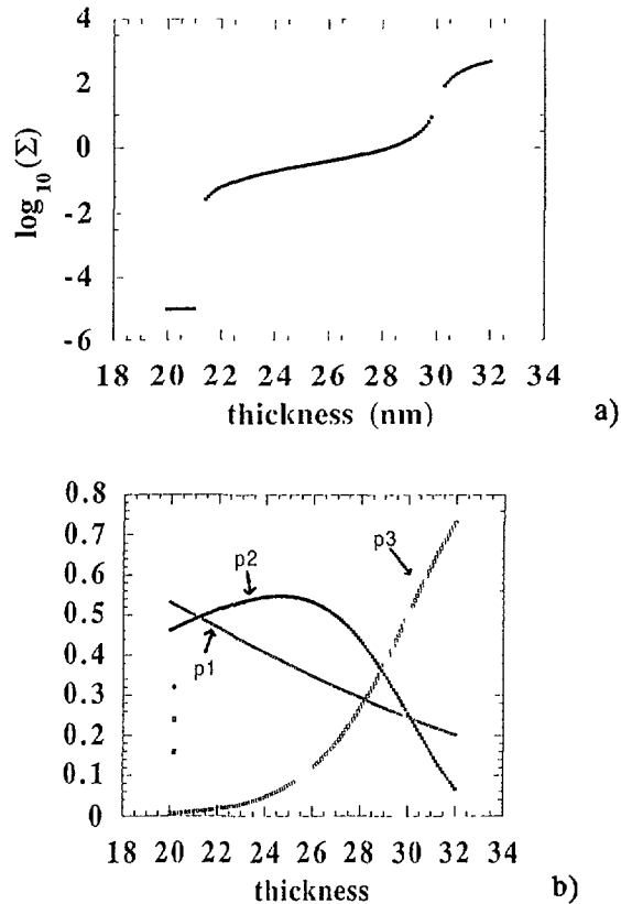
Fig. 2. — a) Conductance versus thickness curve calculated using the EMA approximation. The conductivity before 21 nm has arbitrarily been fixed at 10^{-5} S.cm ^{-1} . The figure 2b shows the evolution of p_1 , p_2 and p_3 . The following values have been assumed in equation (5): \epsilon_1 = 21 , \epsilon_3 = 30 , w_1 = 8 and w_3 = 2 .
