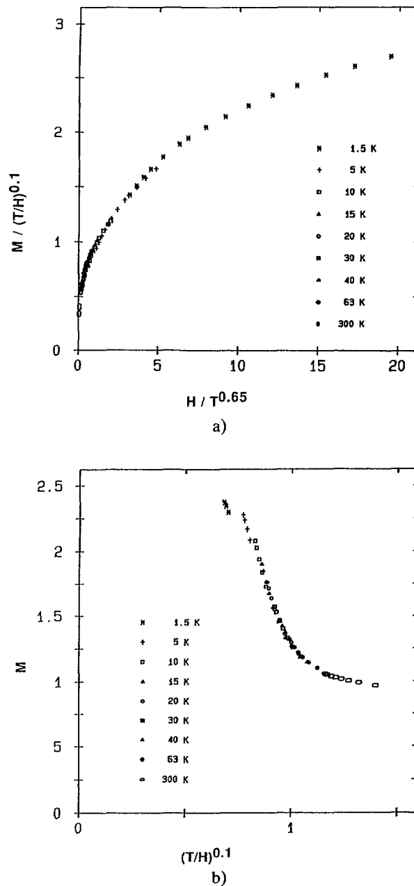
Fig. 4. — Scaling plots of our data points for the low field regime (a) and the large field regime (b).
