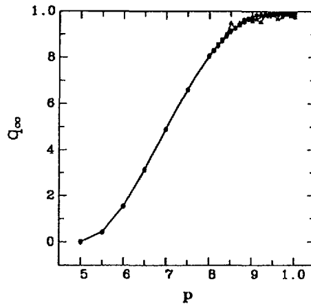
Fig. 1. — Long-time limit of the two-timestep autocorrelation function in dependence of p for N = 512, 1024, 2048 and 8192 .
