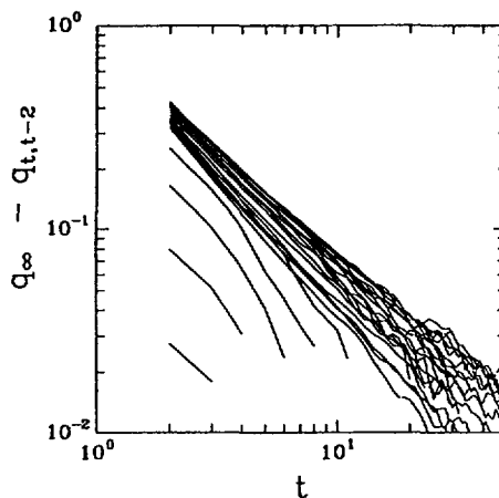
Fig. 2. — Log-log plot of the relaxation behavior of the two-timestep autocorrelation function for different values of p . The t^{-3/2} -behavior is valid for the whole range of \lambda \in [0, 1] .
