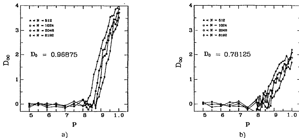
Fig. 5. — Long-time limit D_\infty of the overlap of two configurations with an initial overlap of a) D_0 = 0.97 and b) D_0 = 0.78 and different p and for four different system sizes. The behavior is similar to that of the remanent magnetization.
