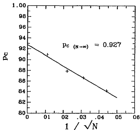
Fig. 4. — The critical value p_c(N) versus 1/\sqrt{N} . The extrapolation yields a limiting value of p_c = 0.93 (i.e. \lambda_c = 0.85 ).
