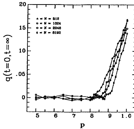
Fig. 3. — Long-time limit of the remanent magnetization versus p for different system sizes.
